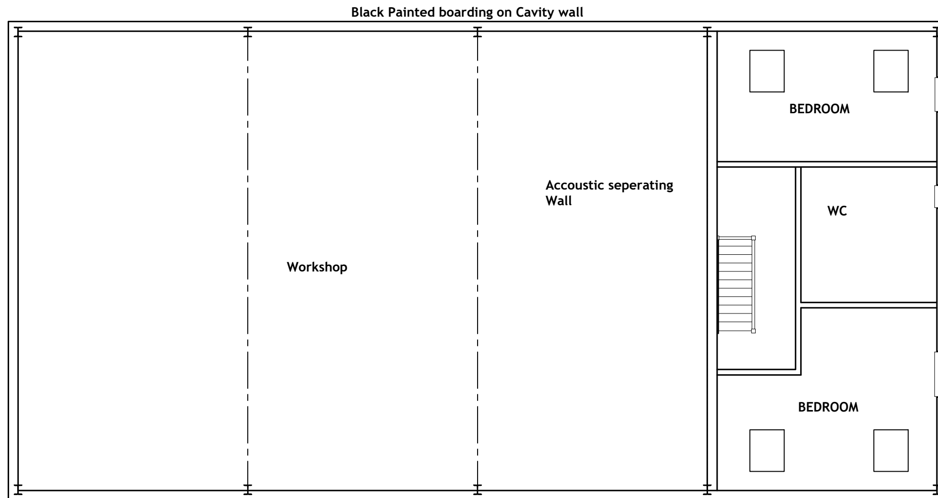
PROPOSED FF PLAN
