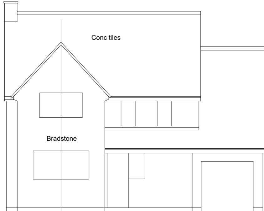
West Elevation (Front)
