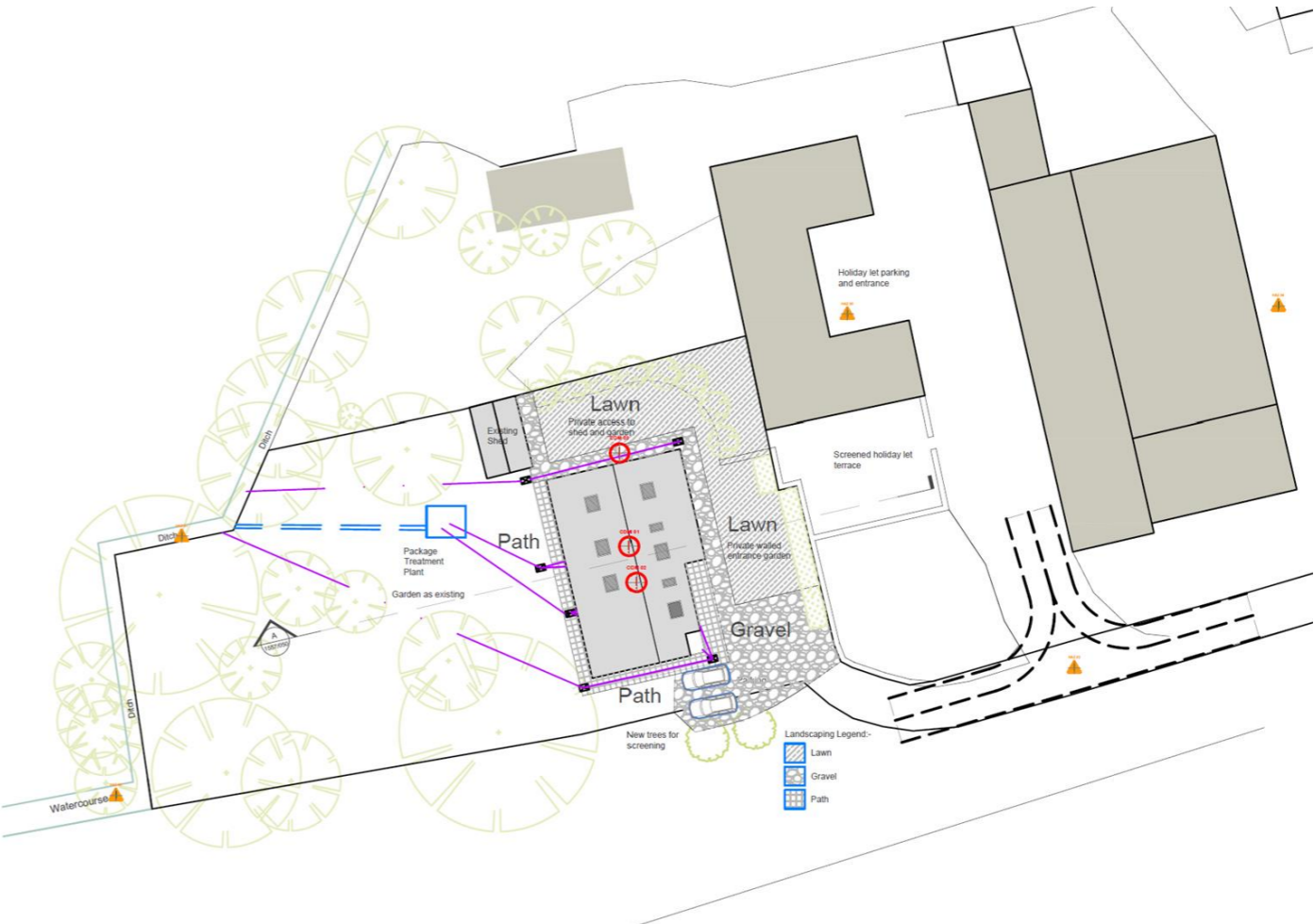
Drawing 1557/100 demonstrating landscape proposals and surface water drainage
