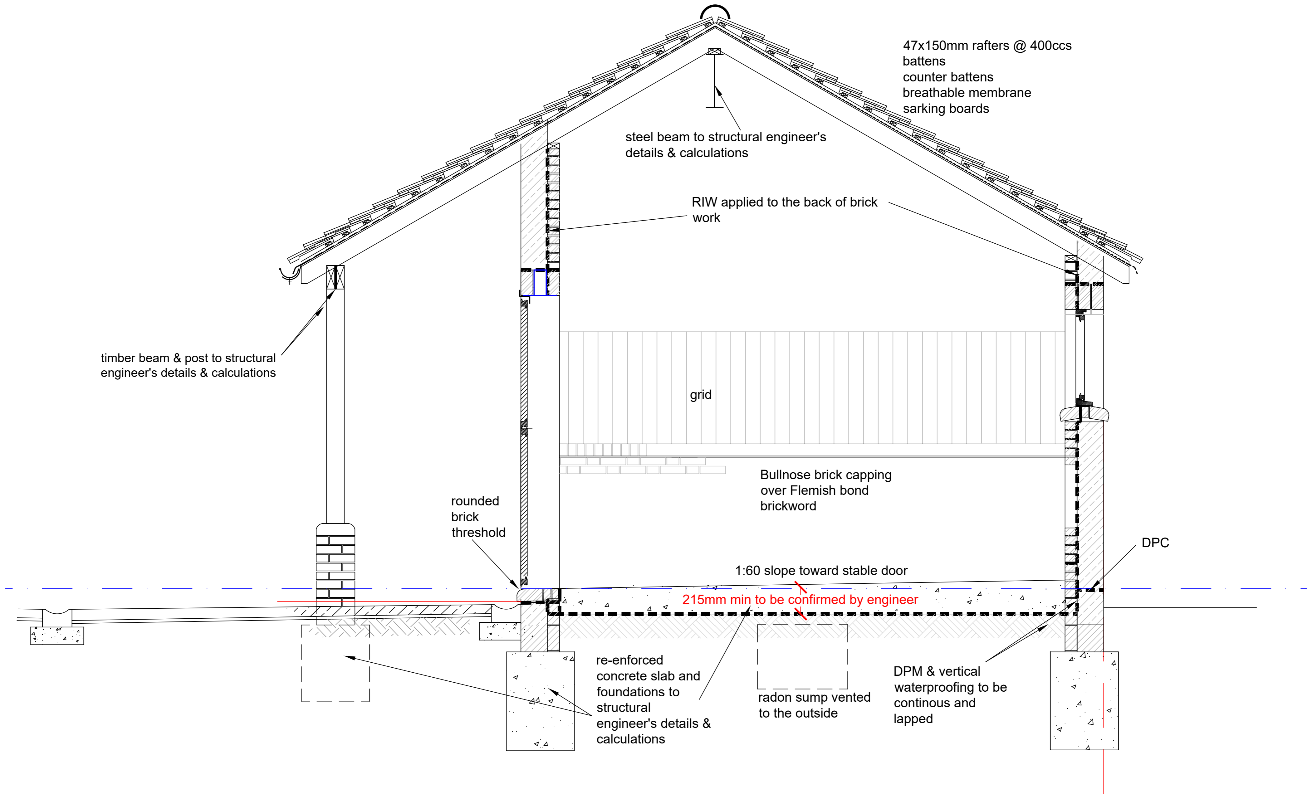
SECTION AA Scale 1/20 @ A2
