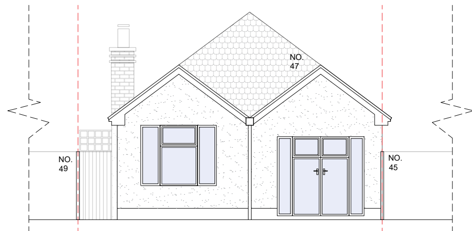
Existing West (Rear) Elevation
