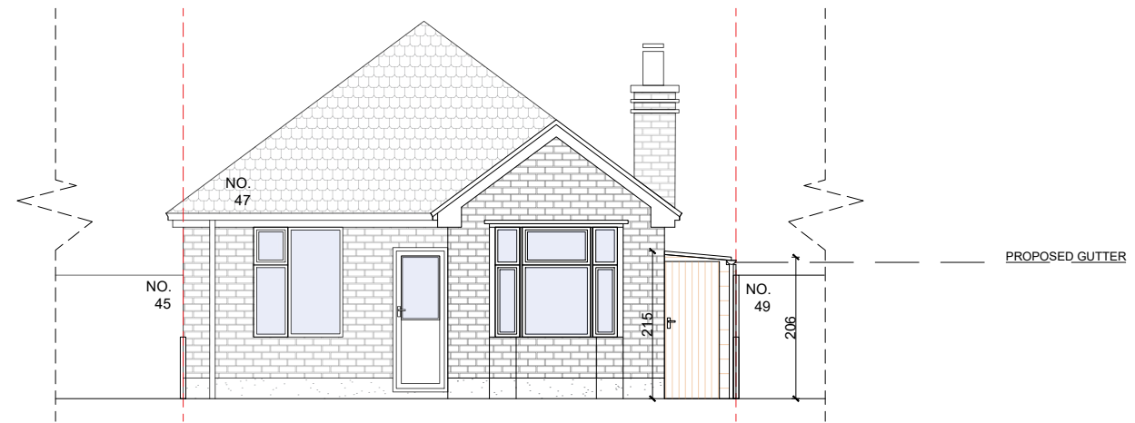
Proposed East (Front) Elevation
