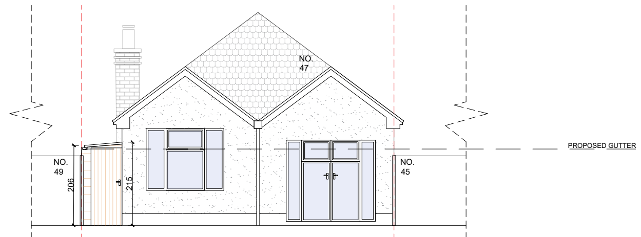
Proposed West (Rear) Elevation
