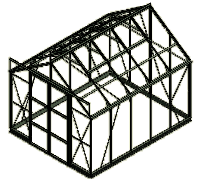
ISOMETRIC VIEW
