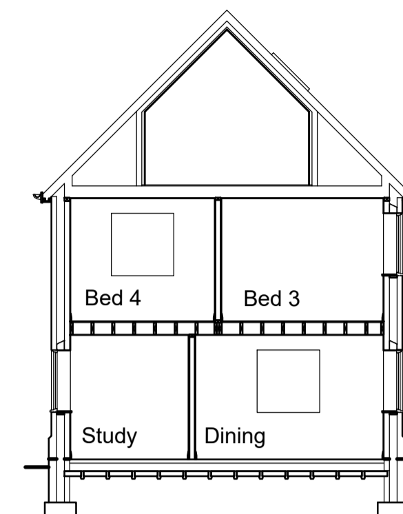
TYPICAL SECTION
