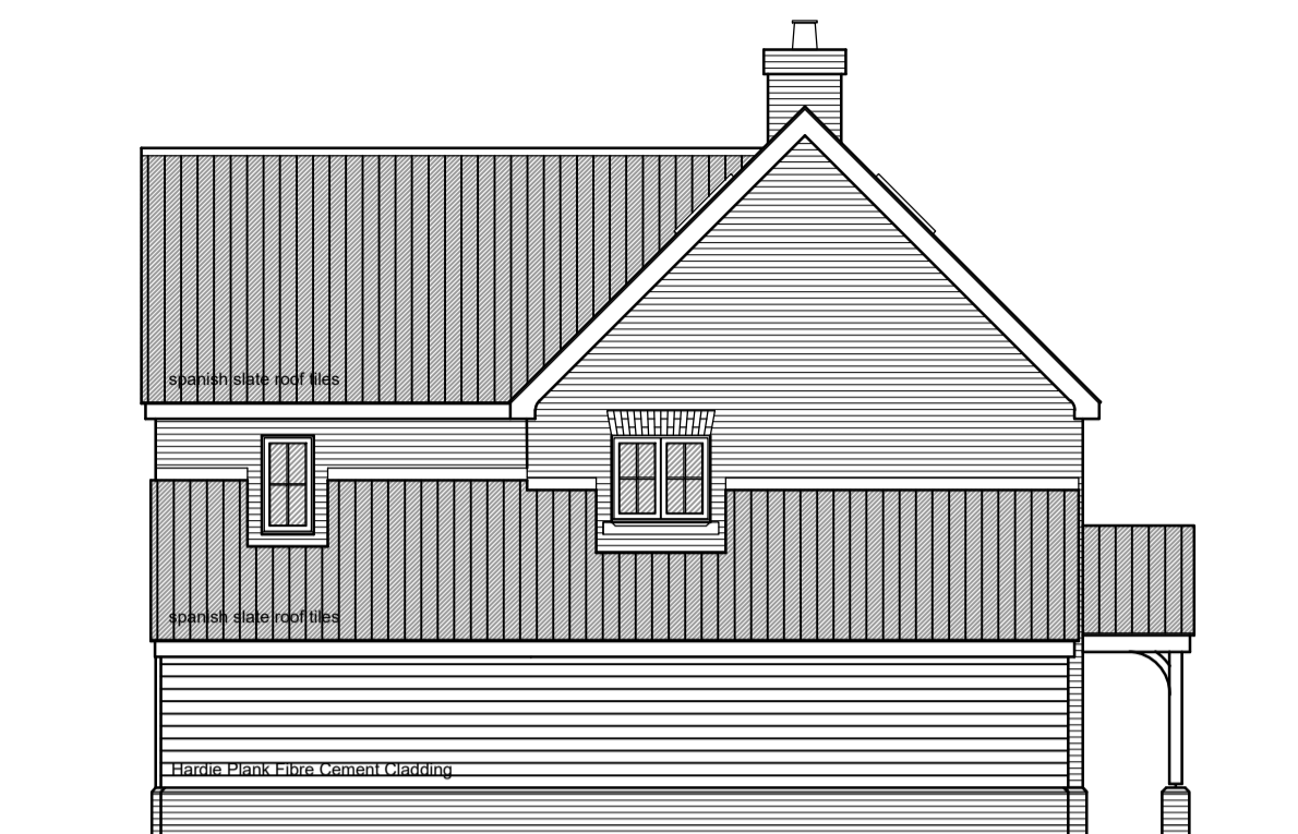
WEST ELEVATION
