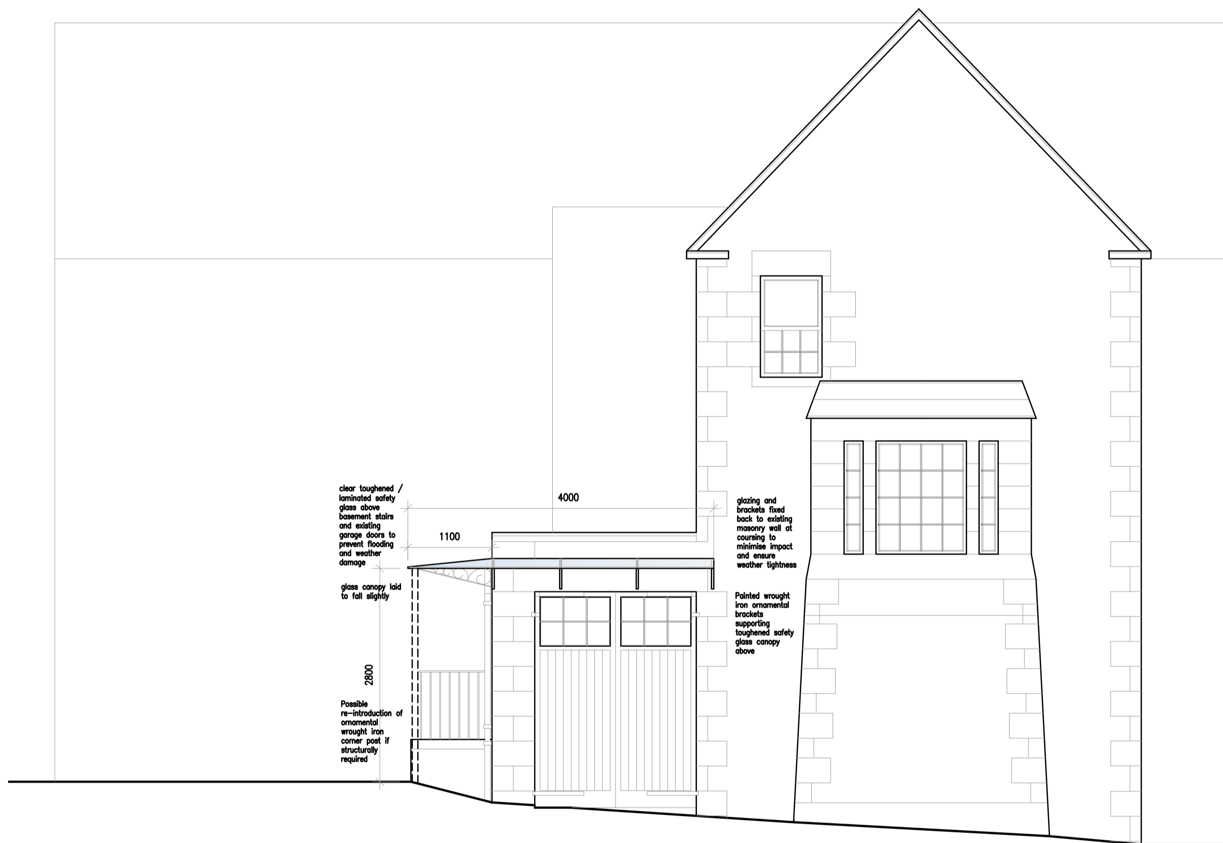
Proposed Main House West Elevation – part (1:50)
