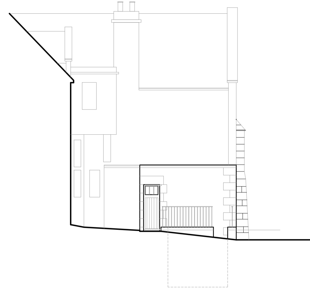
Existing Main House North Elevation – part (1:100)
