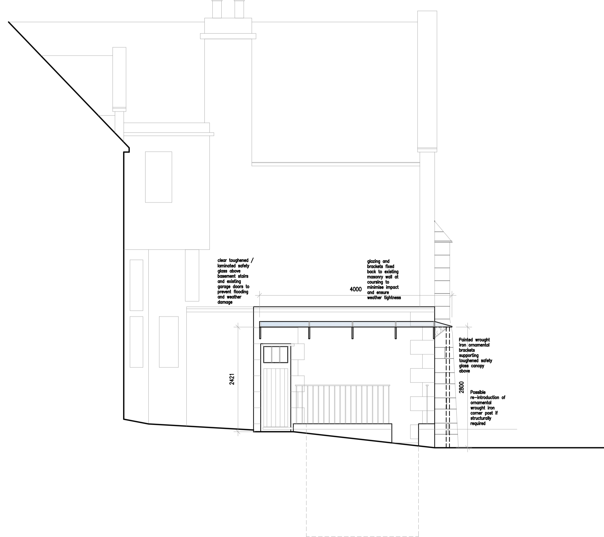
Proposed Main House North Elevation – part (1:50)
