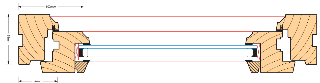
Horizontal Section
