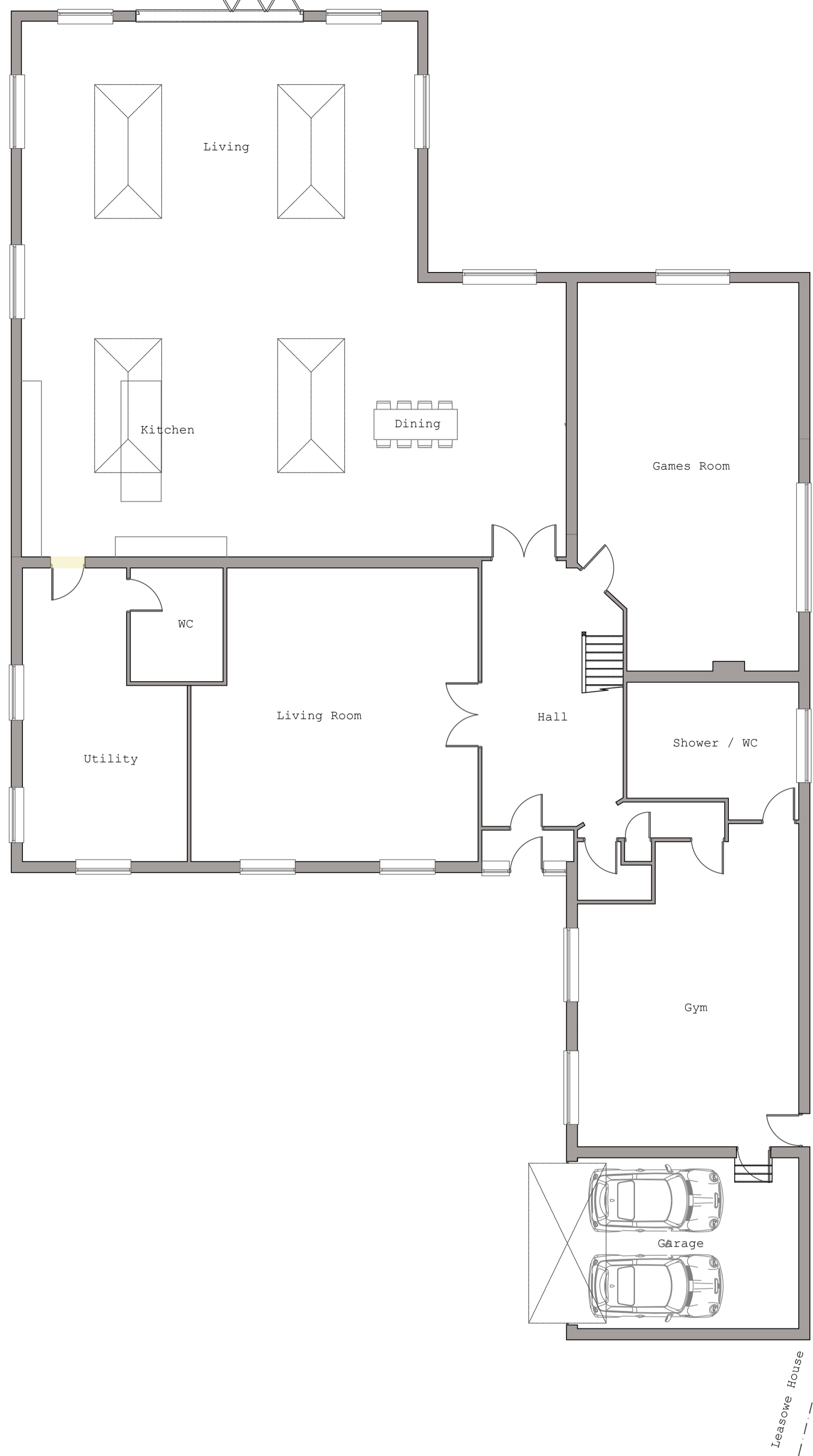
PROPOSED GROUND FLOOR LAYOUT (SCALE 1:100)
