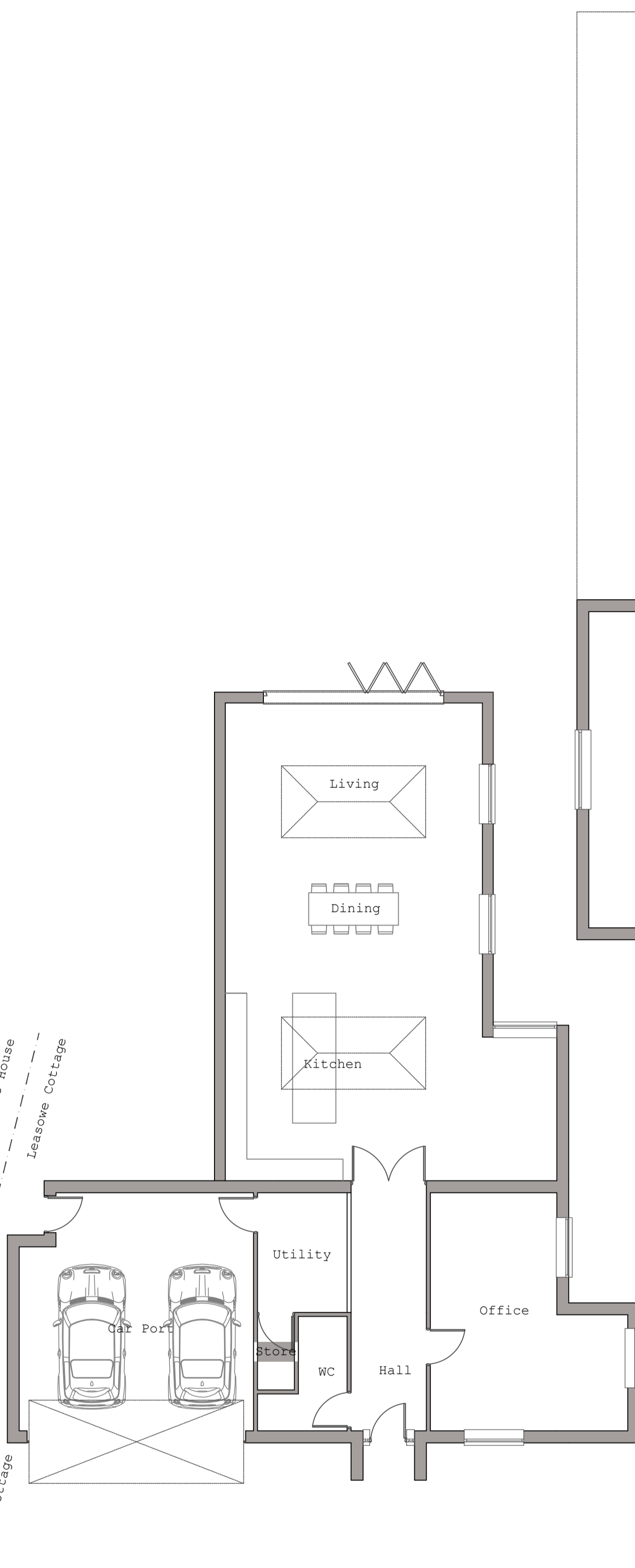
PROPOSED GROUND FLOOR LAYOUT (SCALE 1:100)
