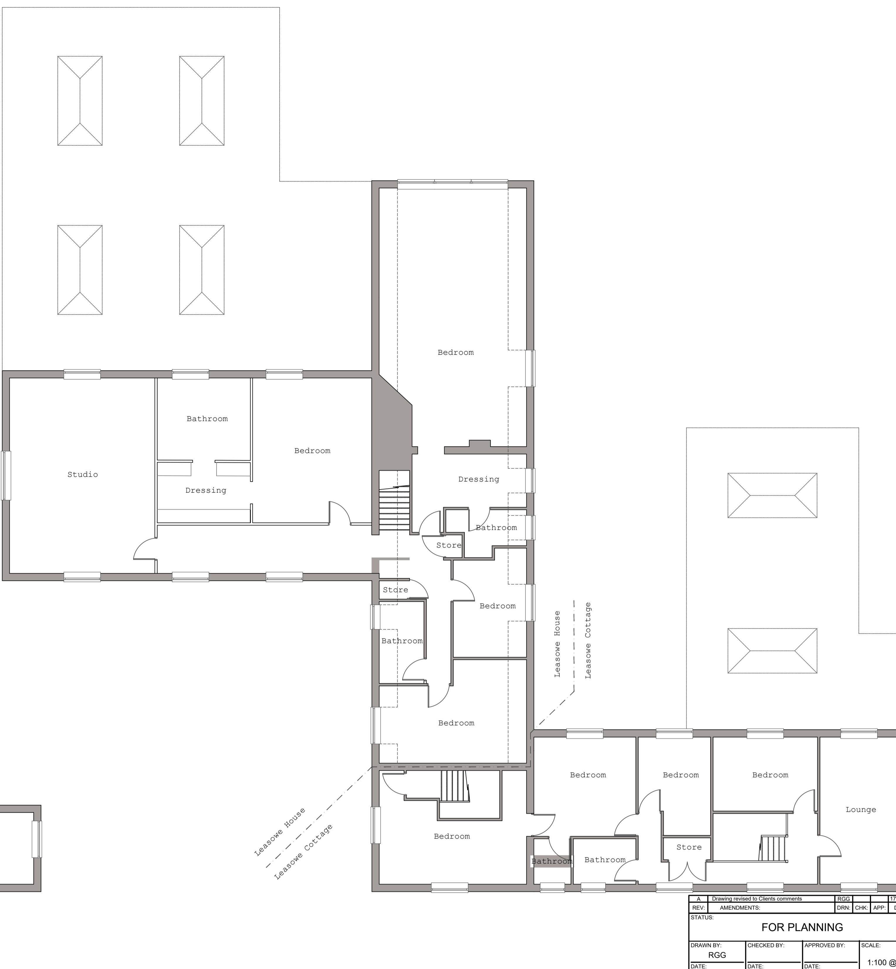
PROPOSED FIRST FLOOR LAYOUT (SCALE 1:100)
