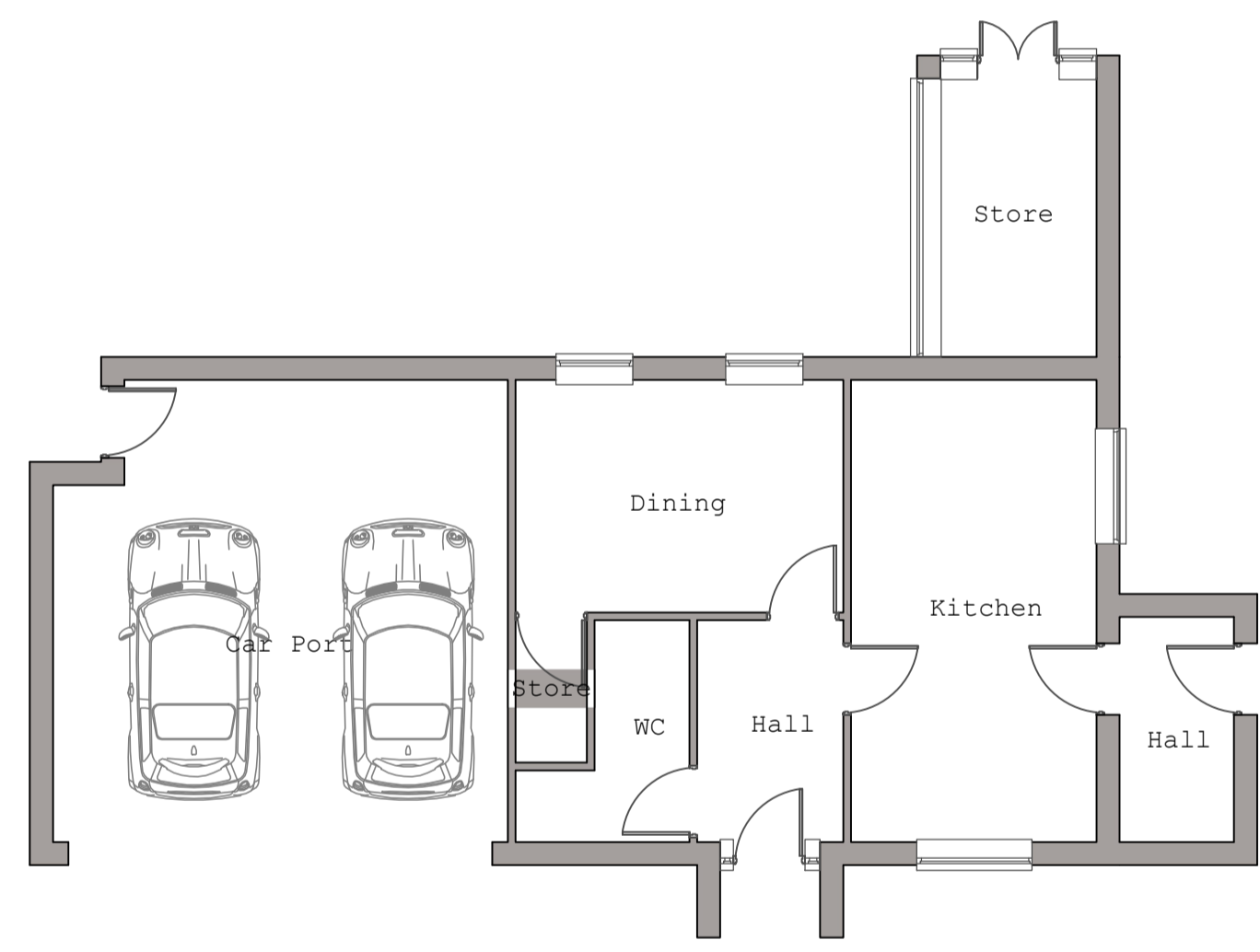
EXISTING GROUND FLOOR LAYOUT (SCALE 1:100)
