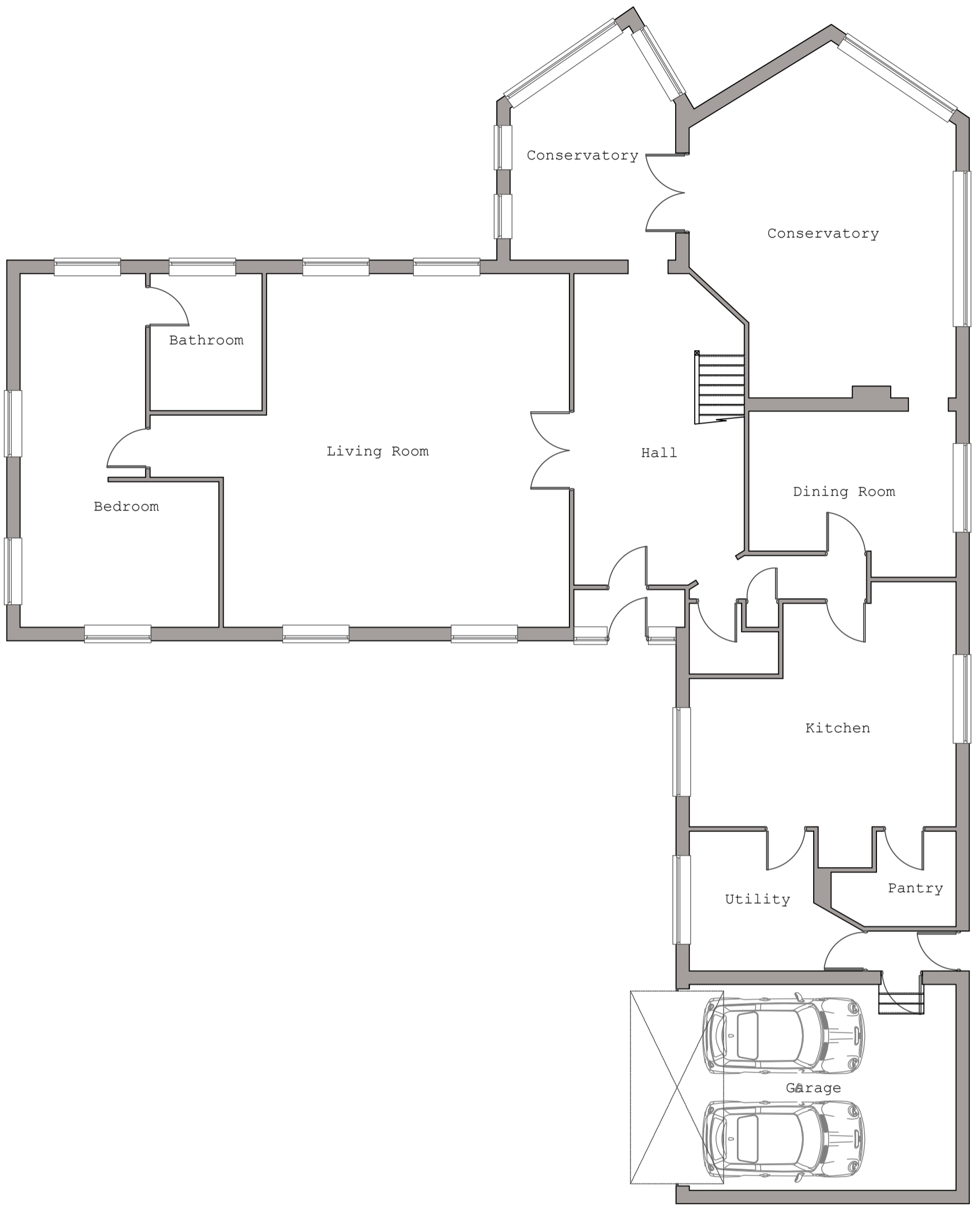
EXISTING GROUND FLOOR LAYOUT (SCALE 1:100)
