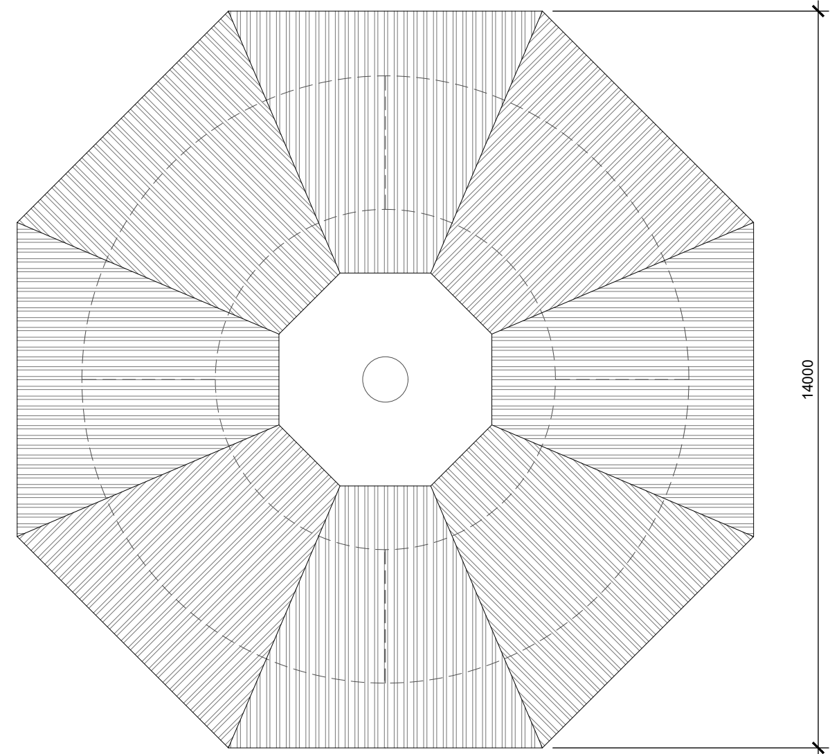
Proposed Horse Walker - Roof Plan
