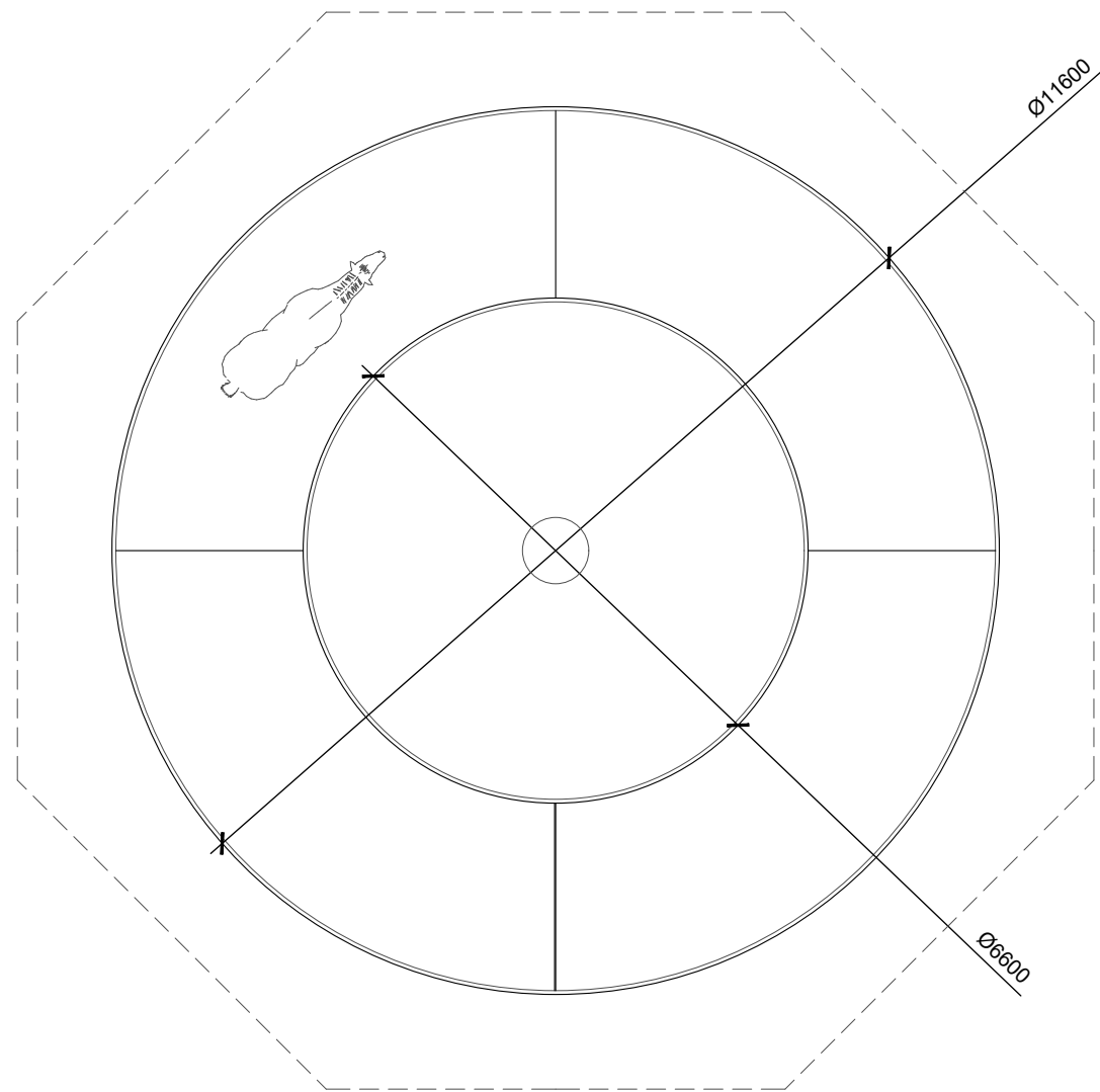
Proposed Horse Walker - Floor Plan
