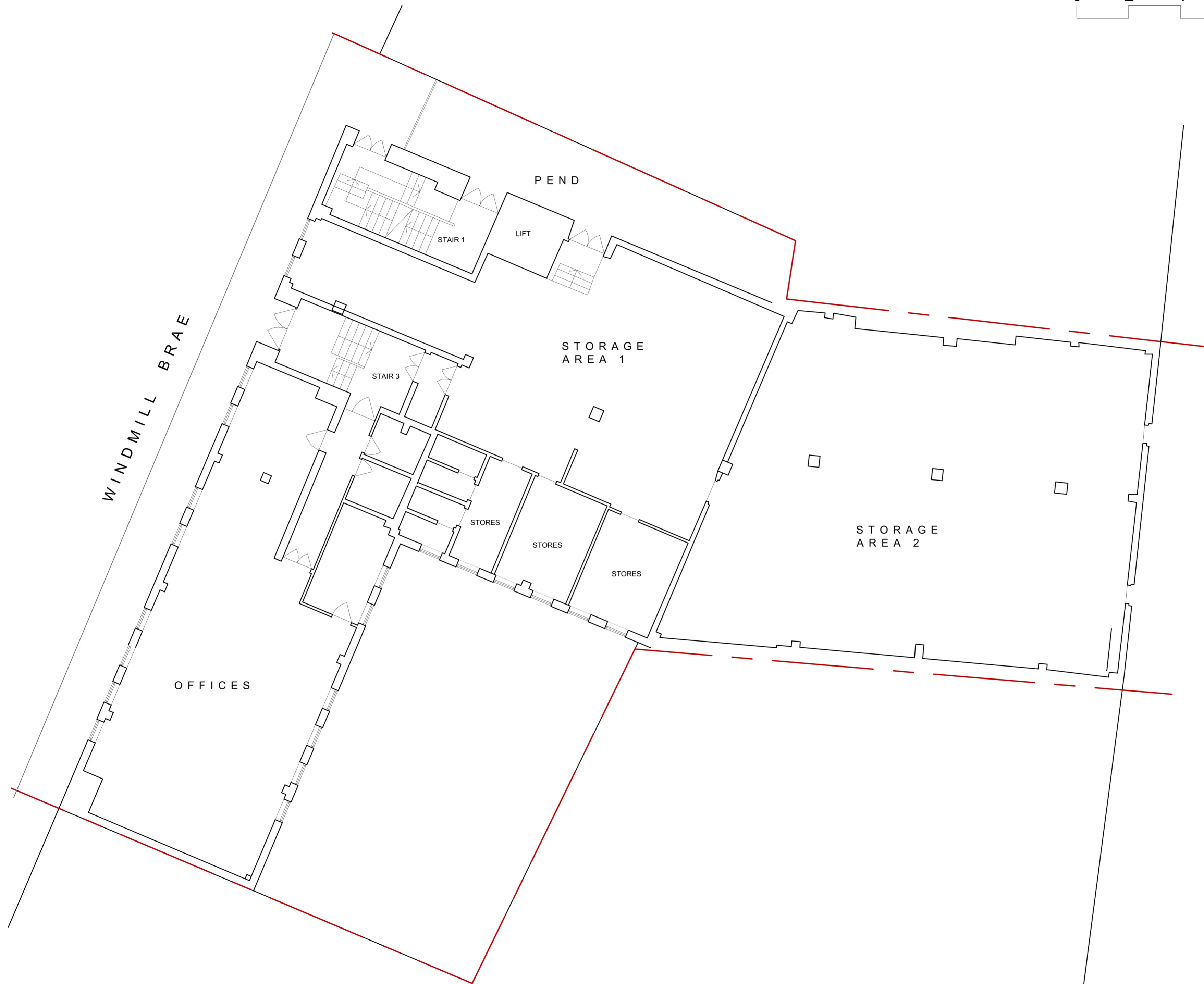
EXISTING LOWER GROUND FLOOR PLAN
