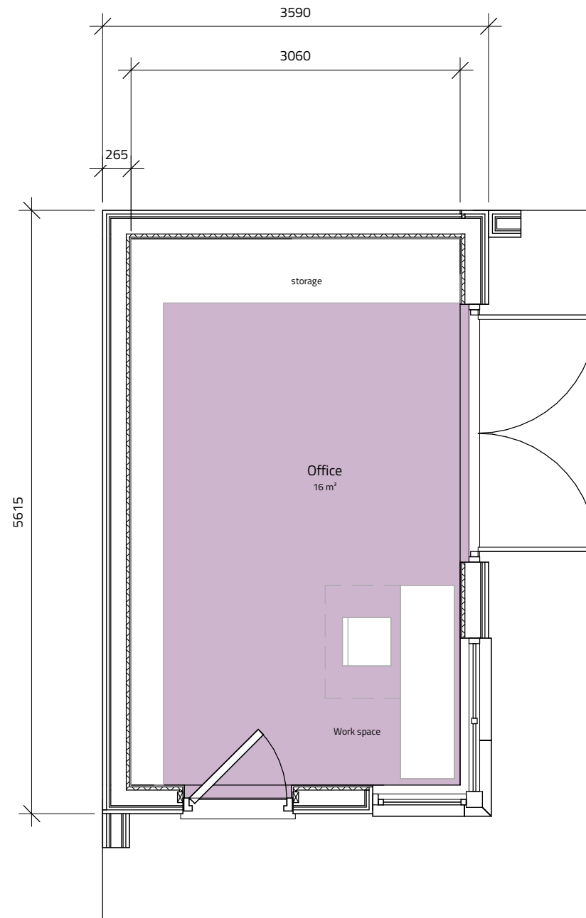
Garden Office - Floor Plan 1 : 50
