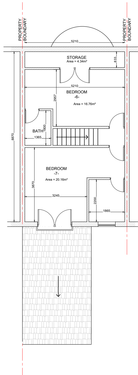
Proposed Loft Plan Scale: 1/100
