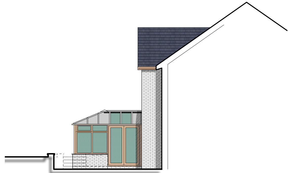
EXISTING PART EAST SIDE SECTION/ELEVATION 1:100 @ A3
