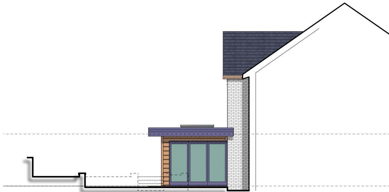
PROPOSED PART EAST SIDE SECTION/ELEVATION 1:100 @ A3
