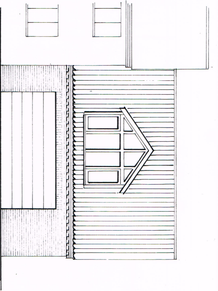
West Elevation
