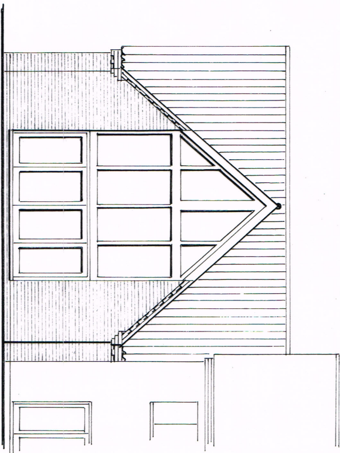
East Elevation
