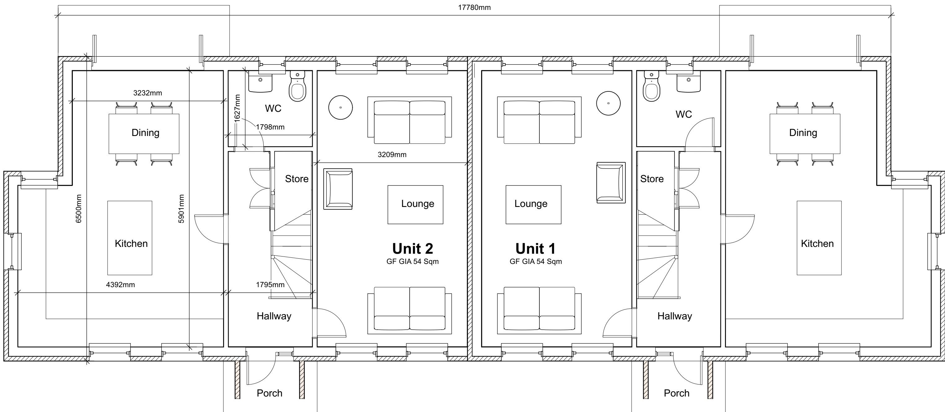
1 Ground Floor Plan Scale: 1:50
