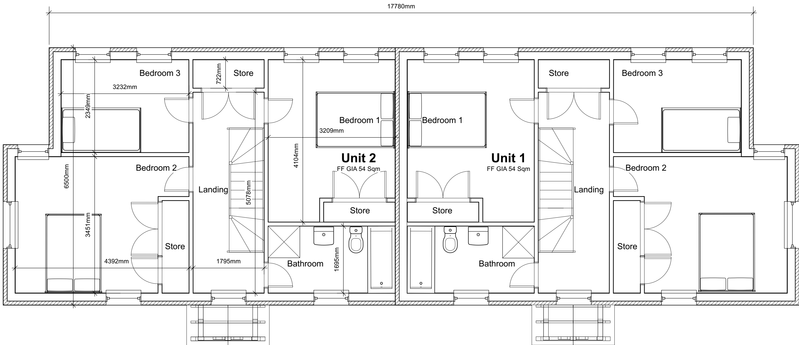
1 First Floor Plan Scale: 1:50
