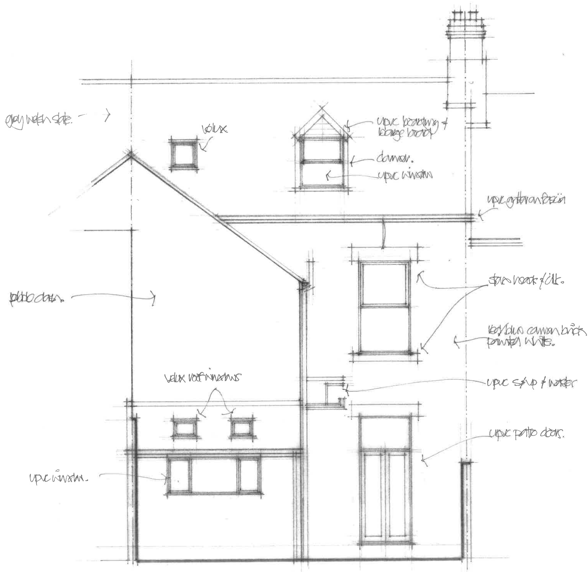
Rear Elevation
