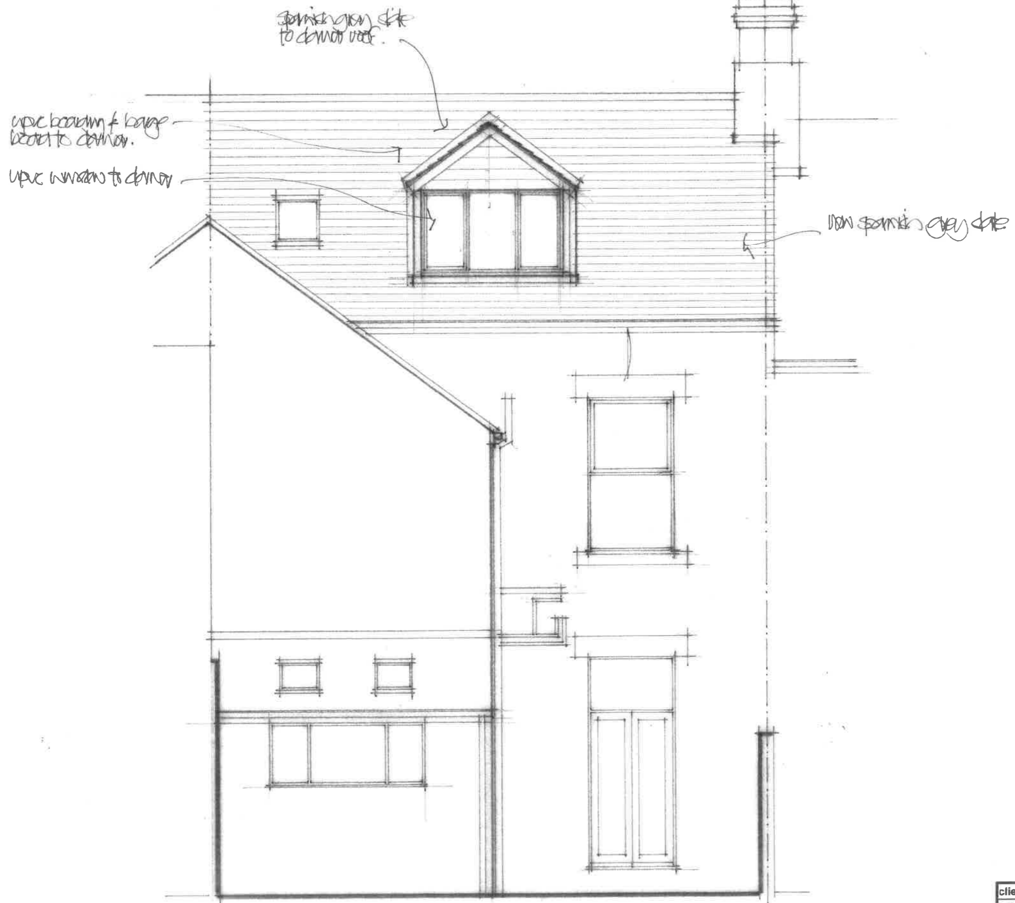
Rear Elevation
