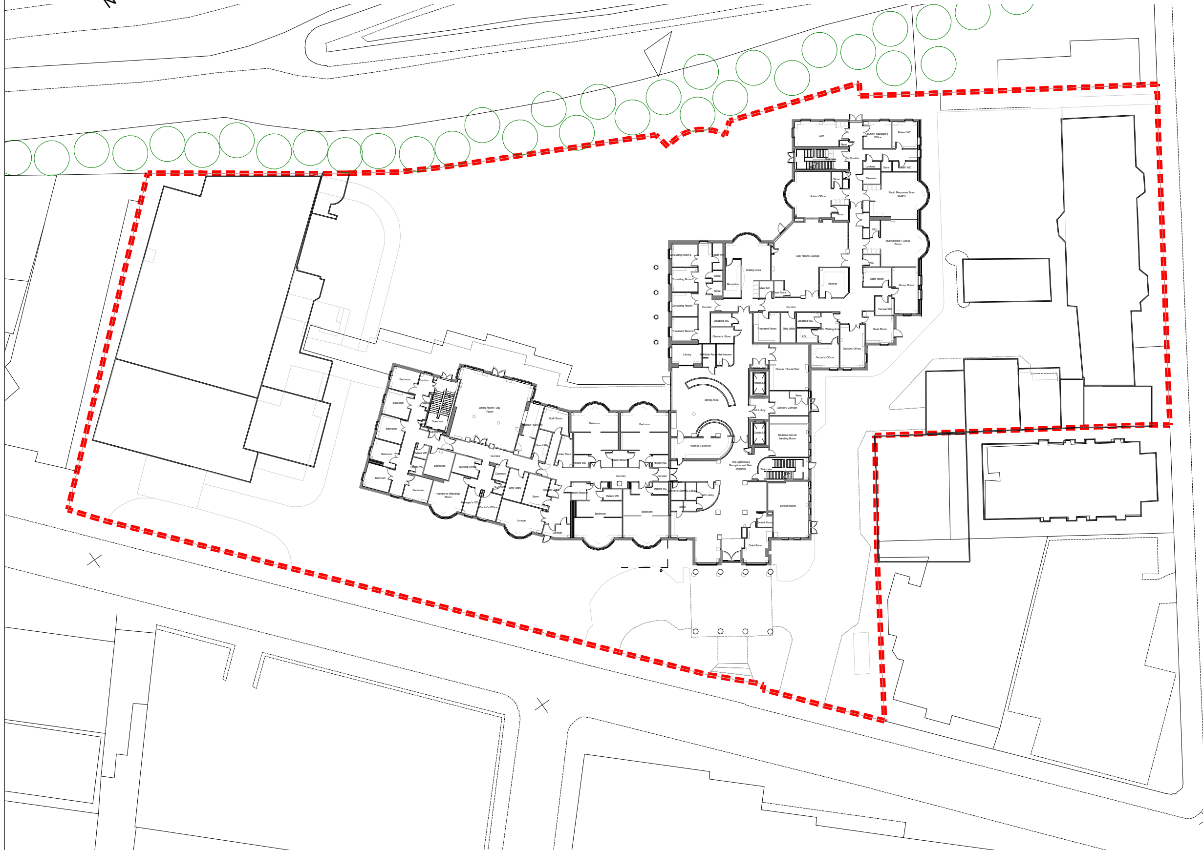
0102 - Existing Ground Floor Plan
