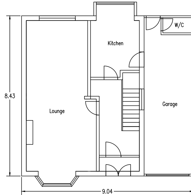
Existing Ground Floor Layout
