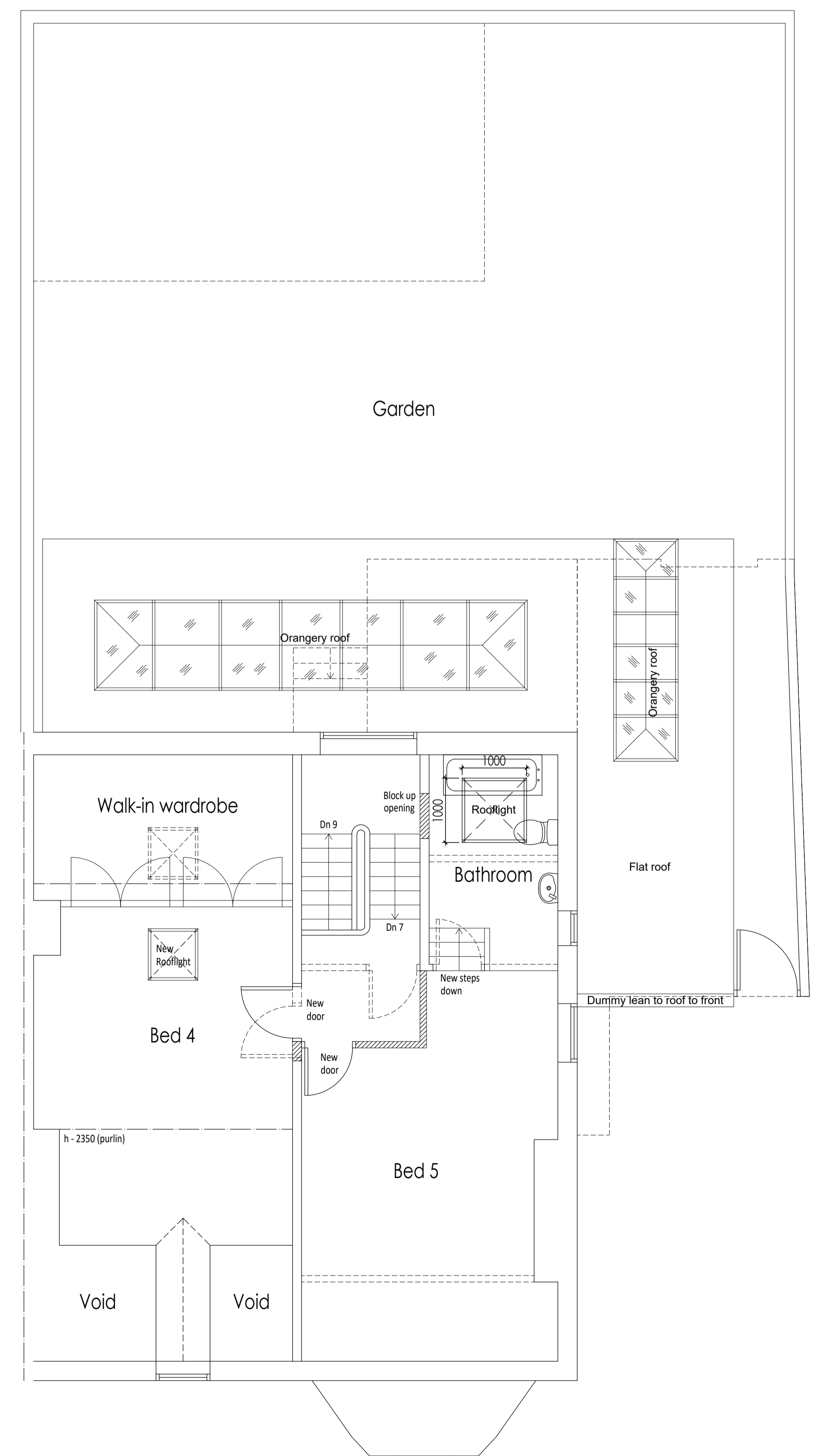
PROPOSED LOFT PLAN
