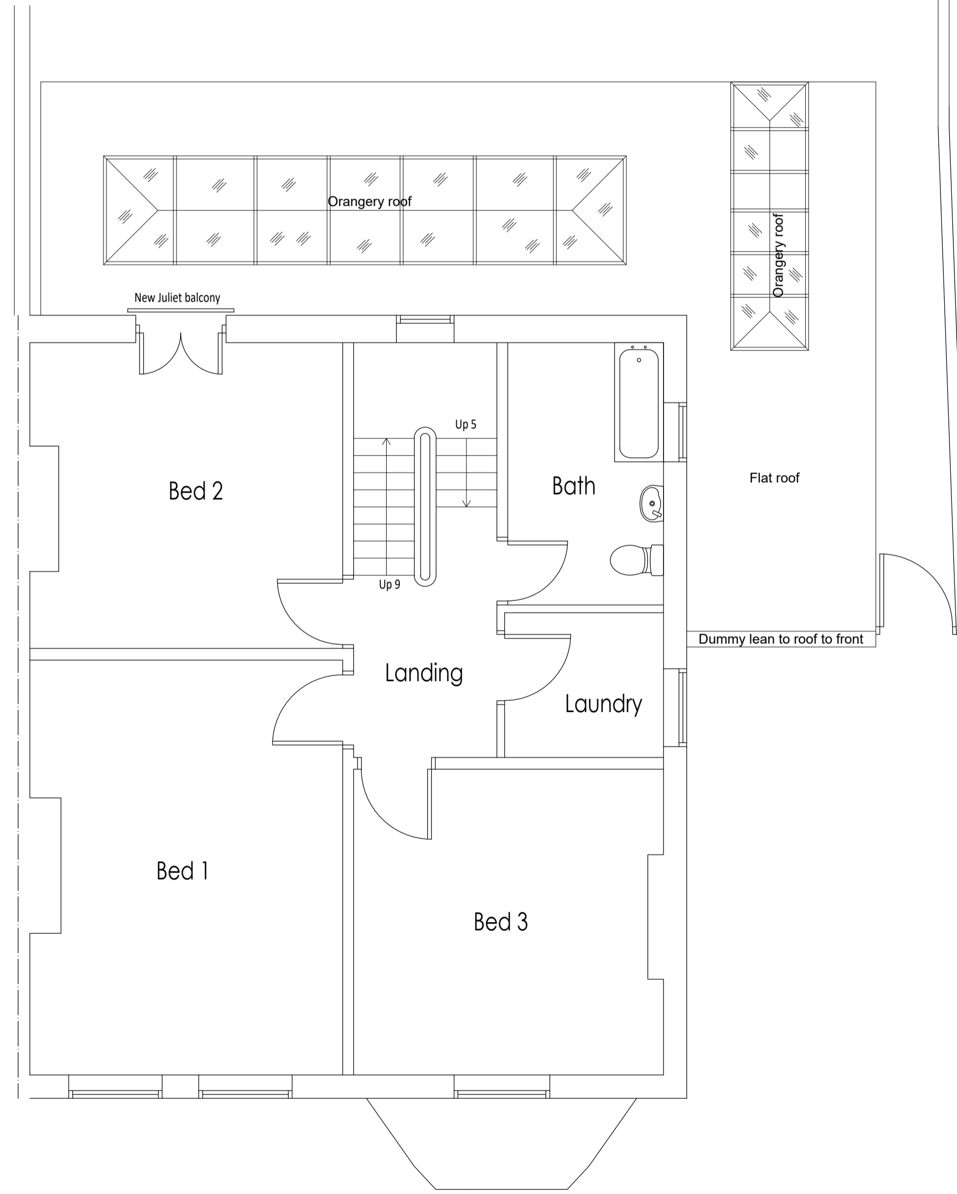
PROPOSED FIRST FLOOR PLAN (not showing demolition)
