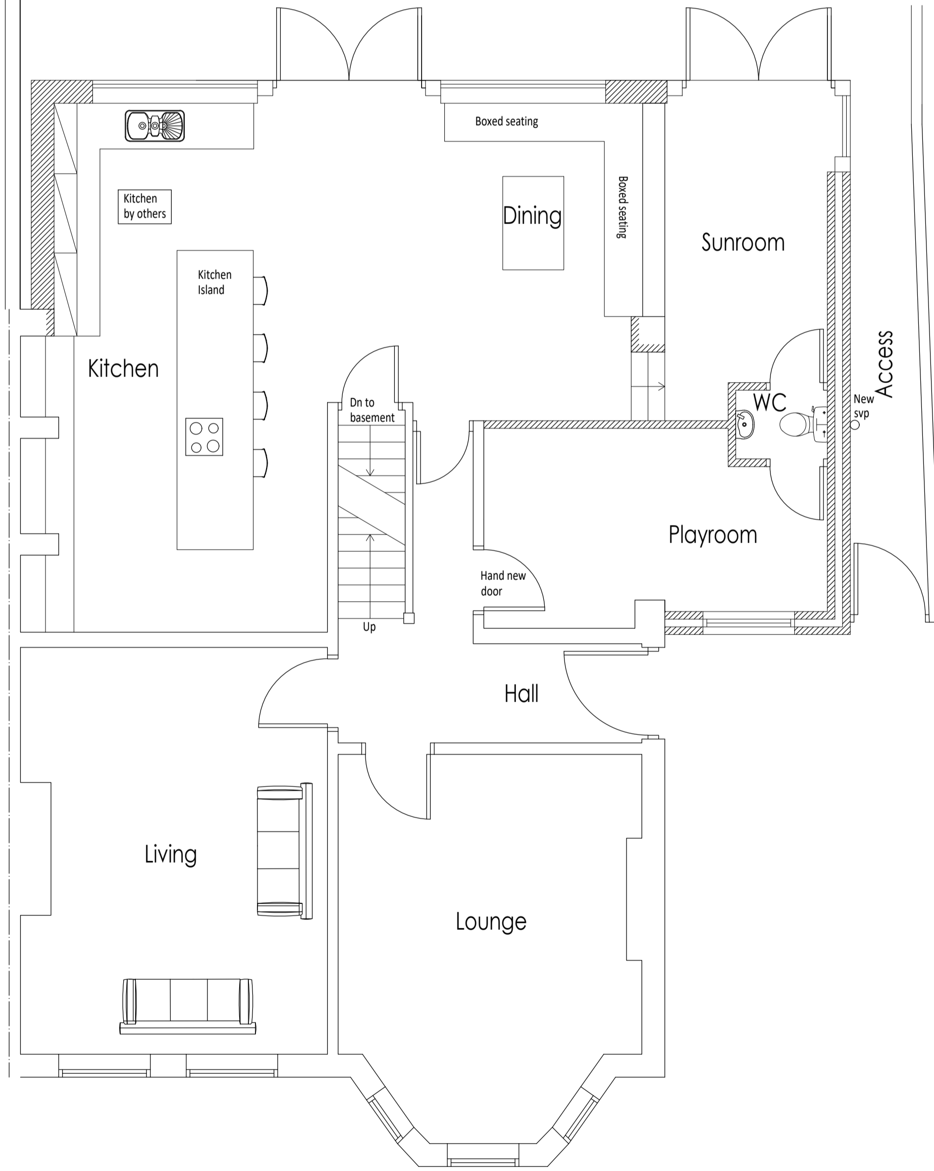
PROPOSED GROUND FLOOR PLAN (not showing demolition)
