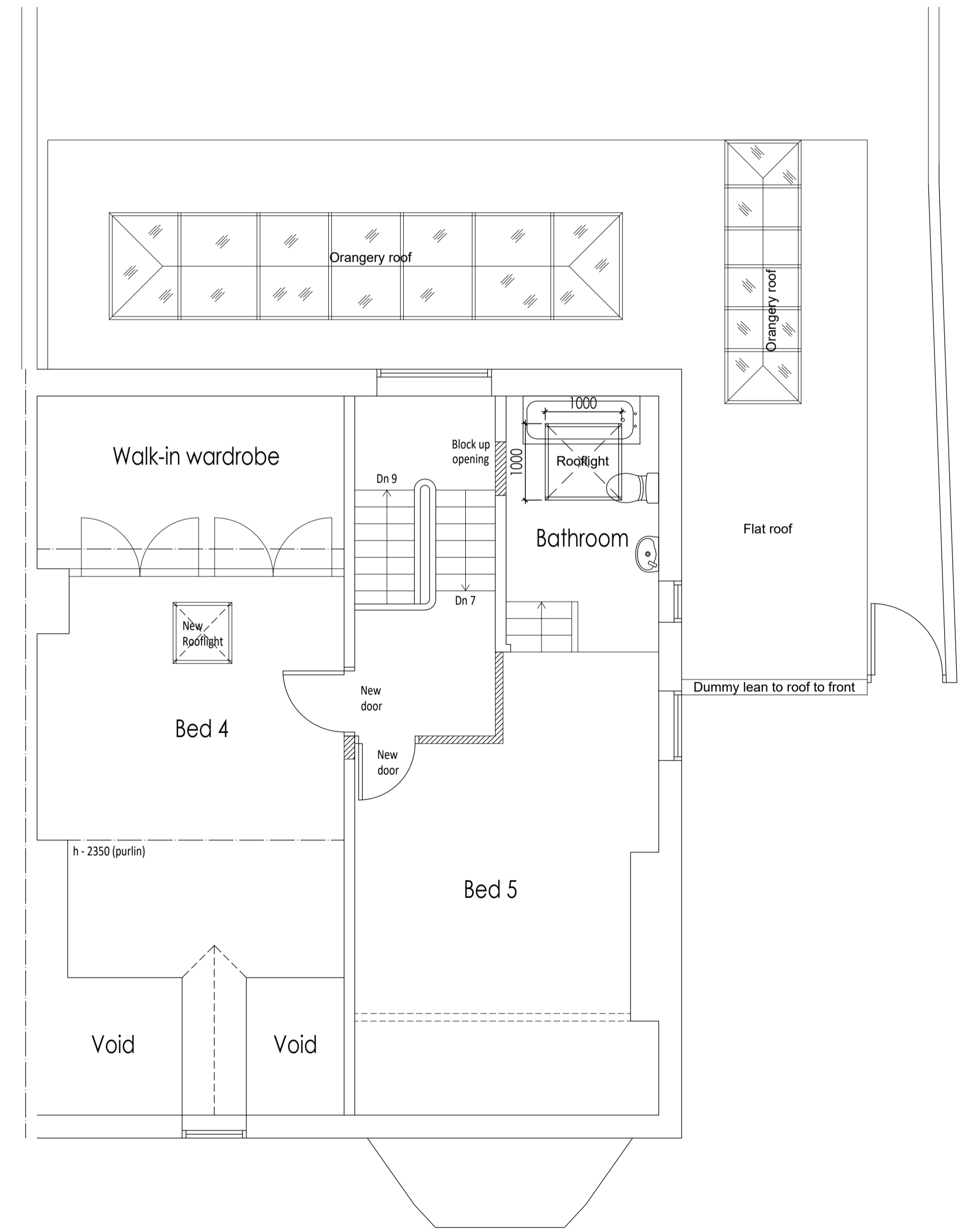
PROPOSED LOFT PLAN (not showing demolition)
