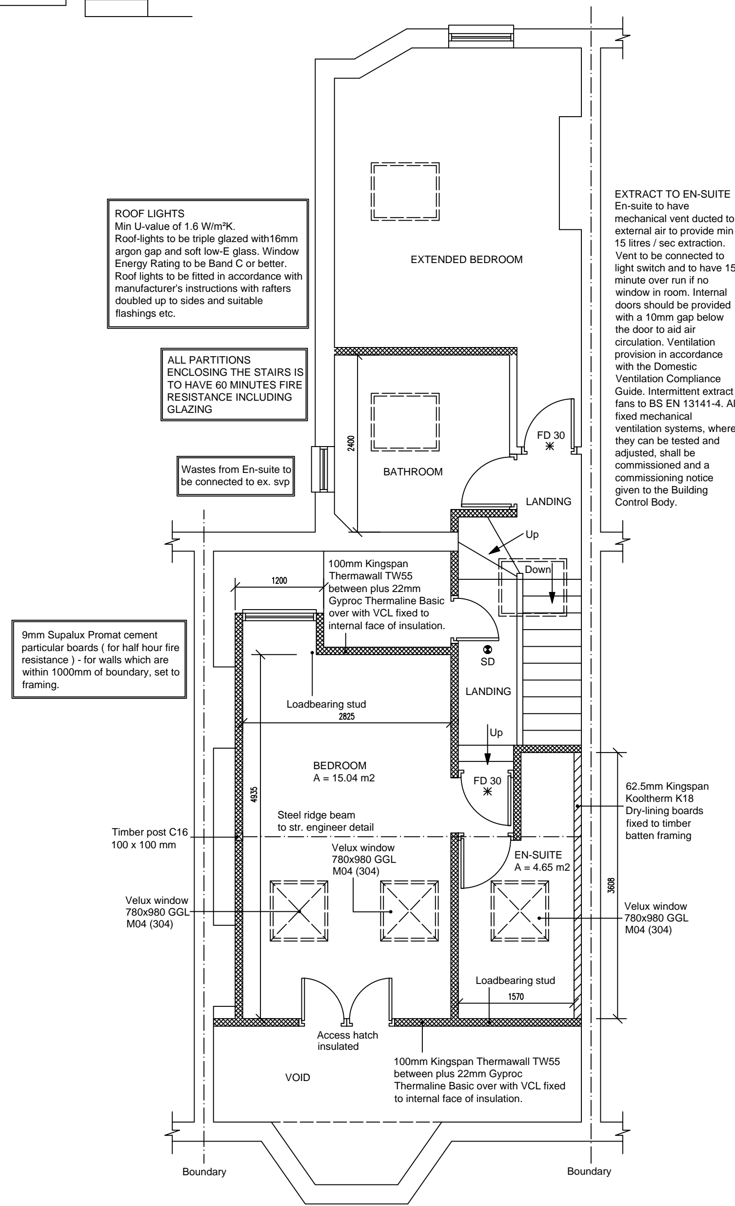
PROPOSED SECOND / ATTIC FLOOR PLAN (scale 1:50)
