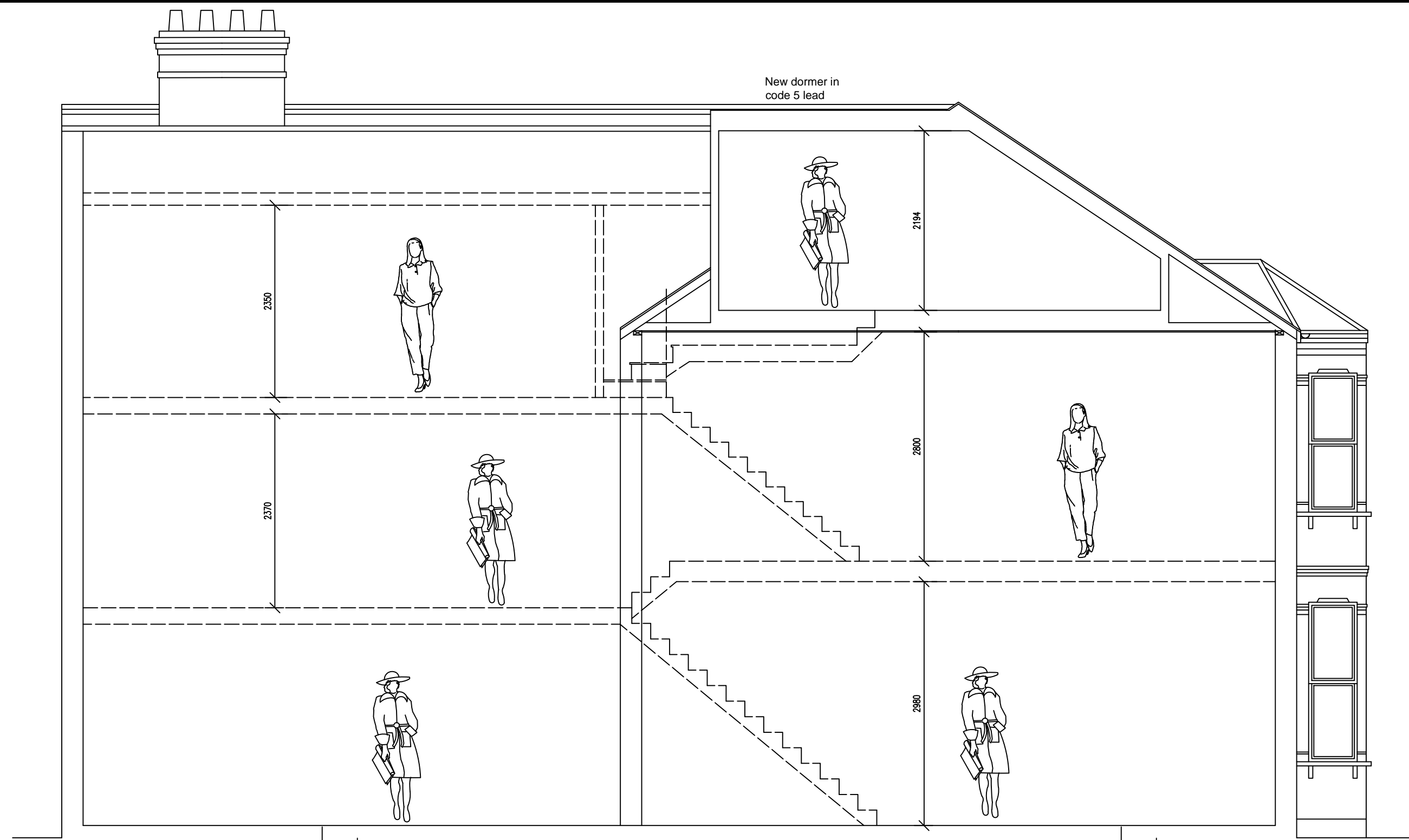
TYPICAL SECTION (scale 1:50)
