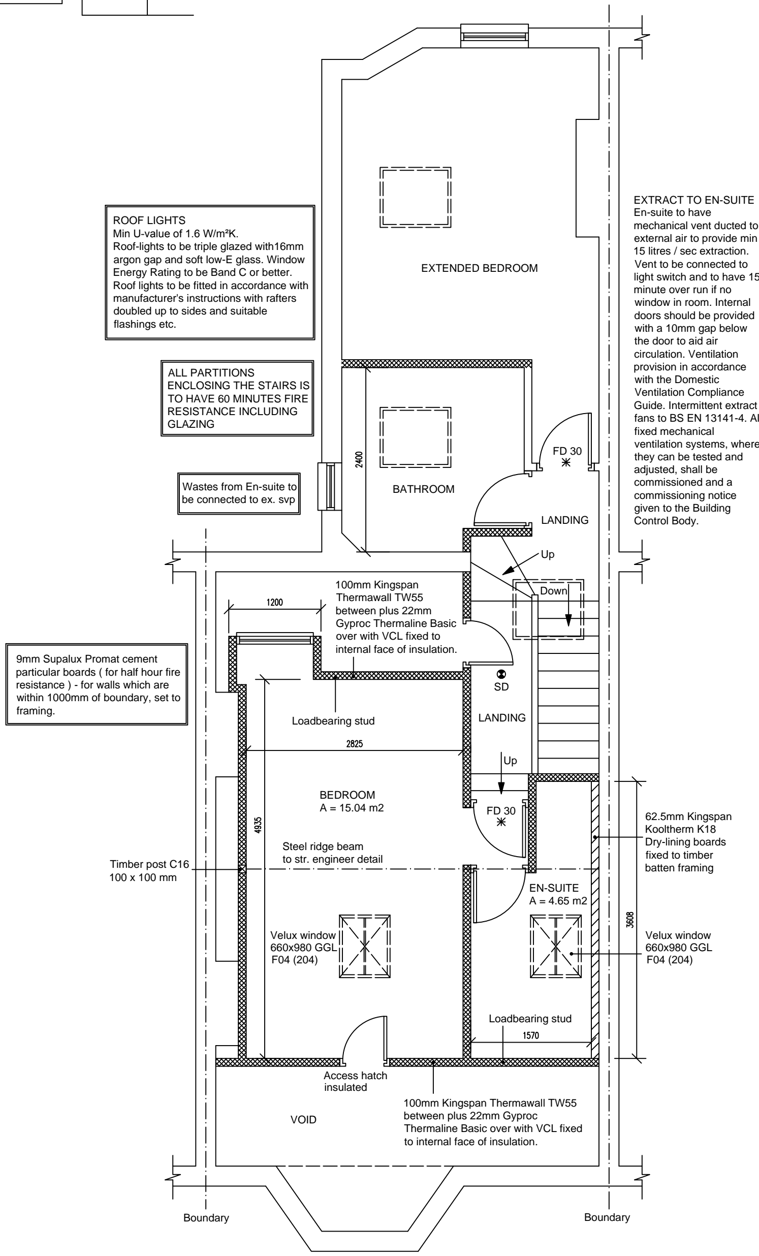
PROPOSED SECOND / ATTIC FLOOR PLAN (scale 1:50)
