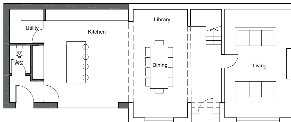
GROUND FLOOR PROPOSED
