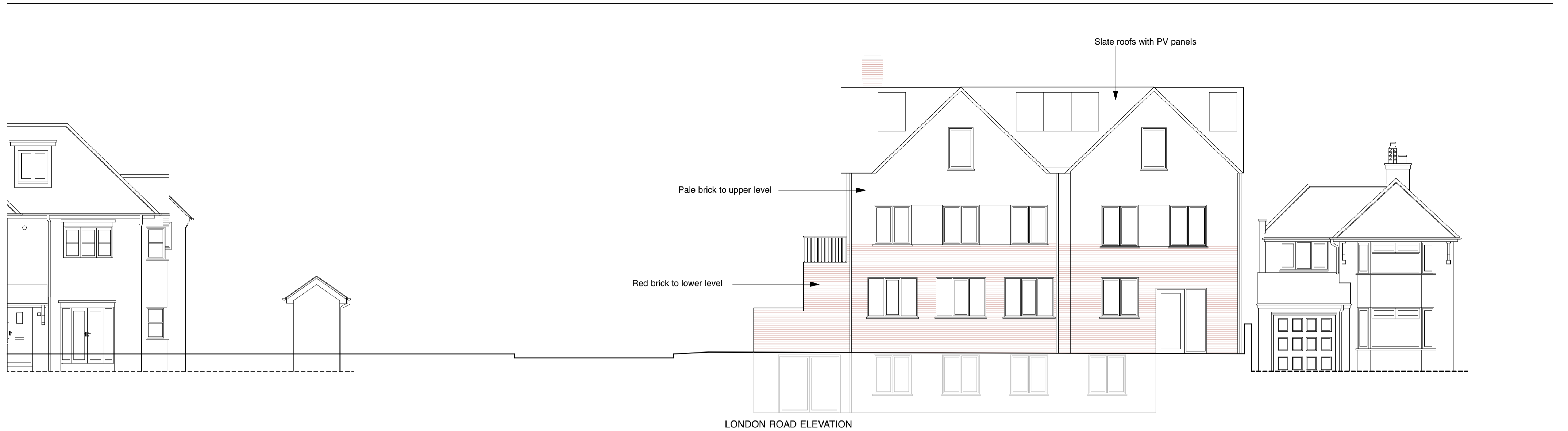
LONDON ROAD ELEVATION
