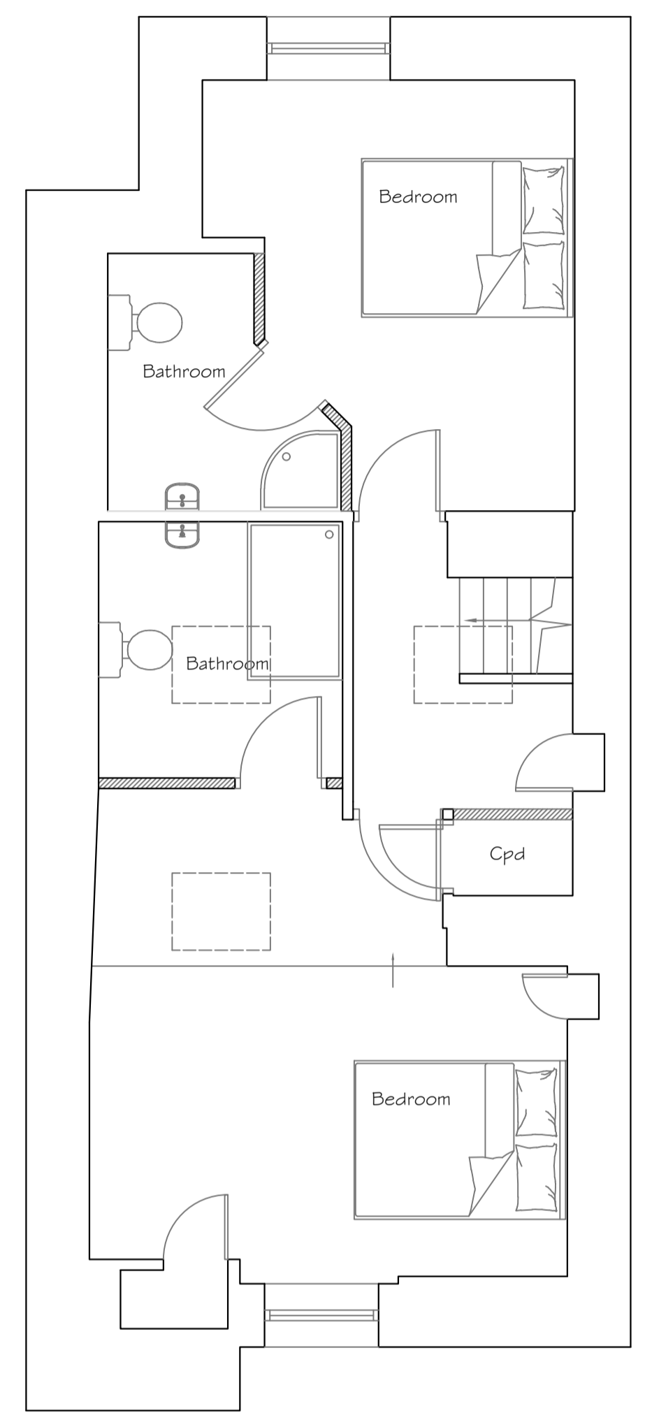
First Floor
