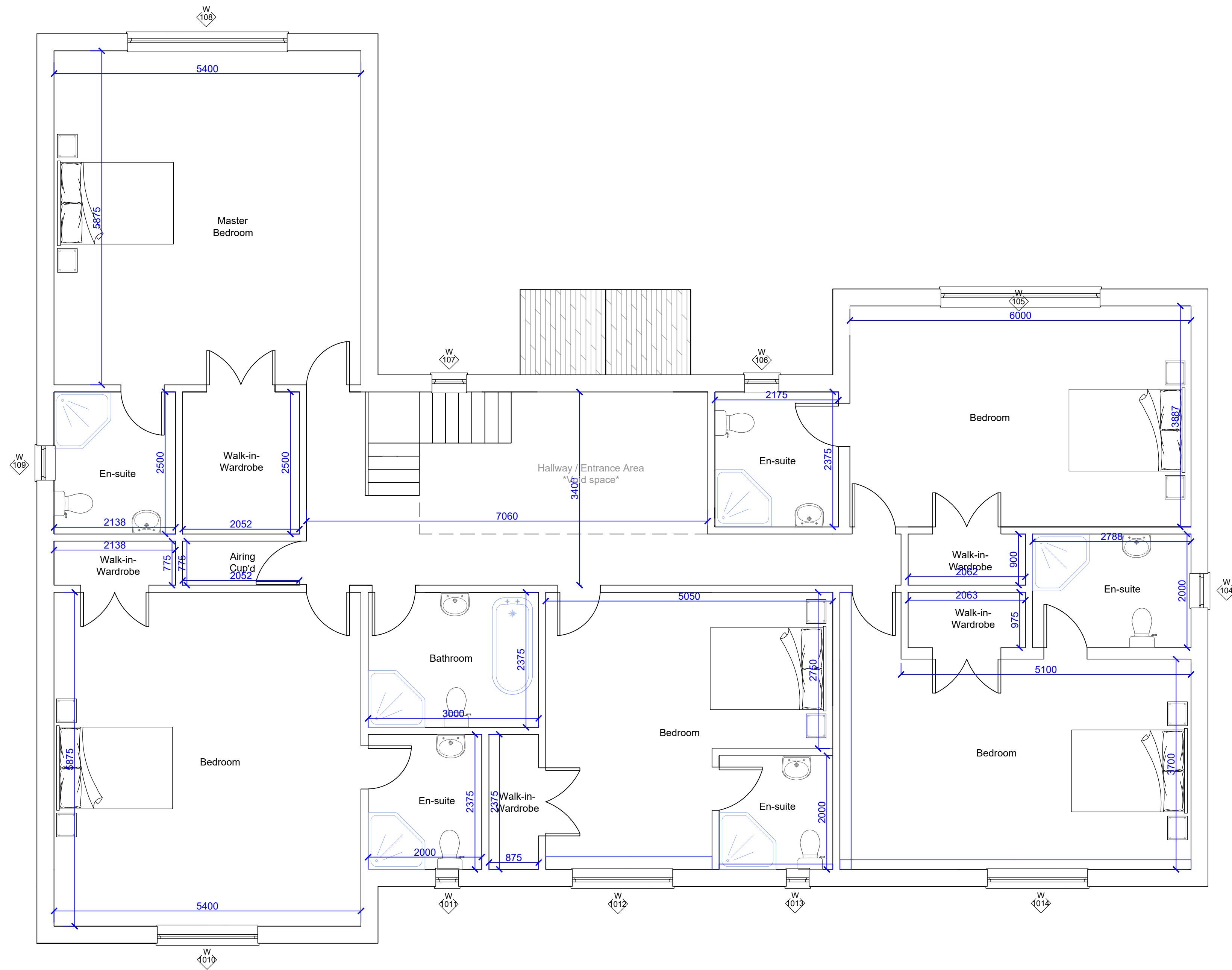
First Floor Plan Scale 1:50
