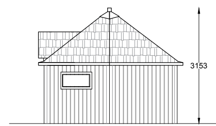
EXISTING RIGHT ELEVATION
