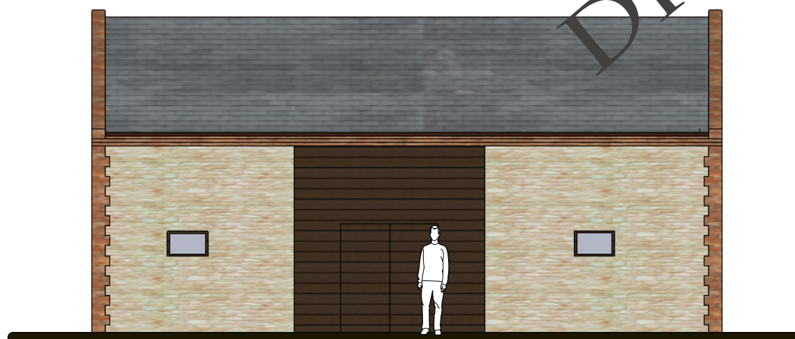
A 16 Front Elevation 1:100
