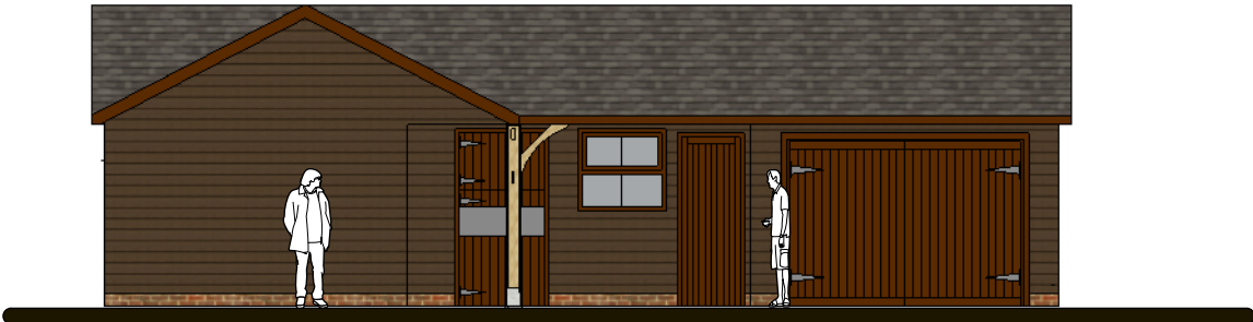
A 8 Side Elevation 1:100
