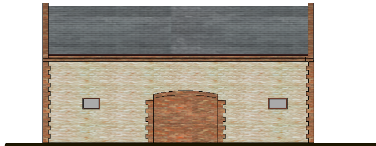
A 17 Rear Elevation 1:100
