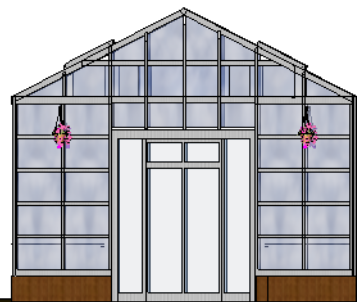
A 19 Rear Elevation 1:100
