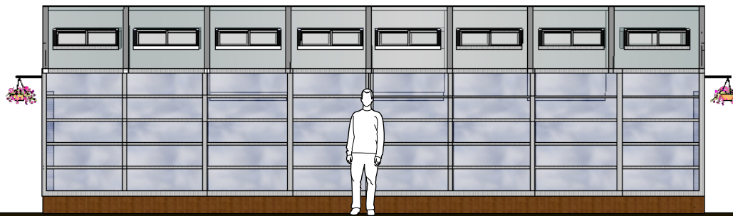
A 21 Side Elevation 1:100
