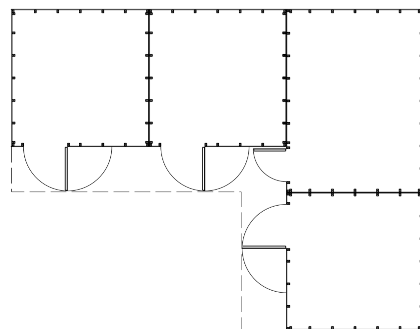
FLOOR PLAN
