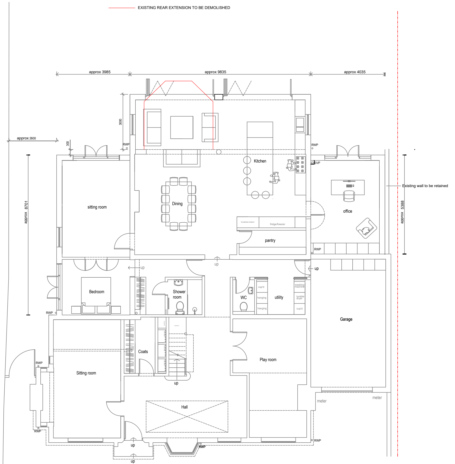
GROUND FLOOR PLAN AS PROPOSED
