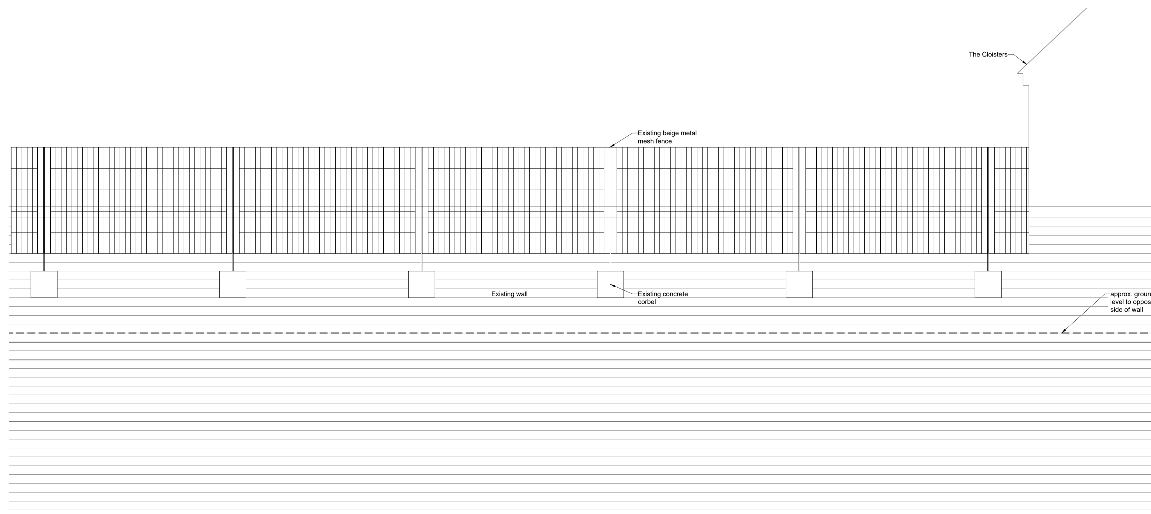
Existing Boundary Fence Elevation from inside the site Scale 1:20
