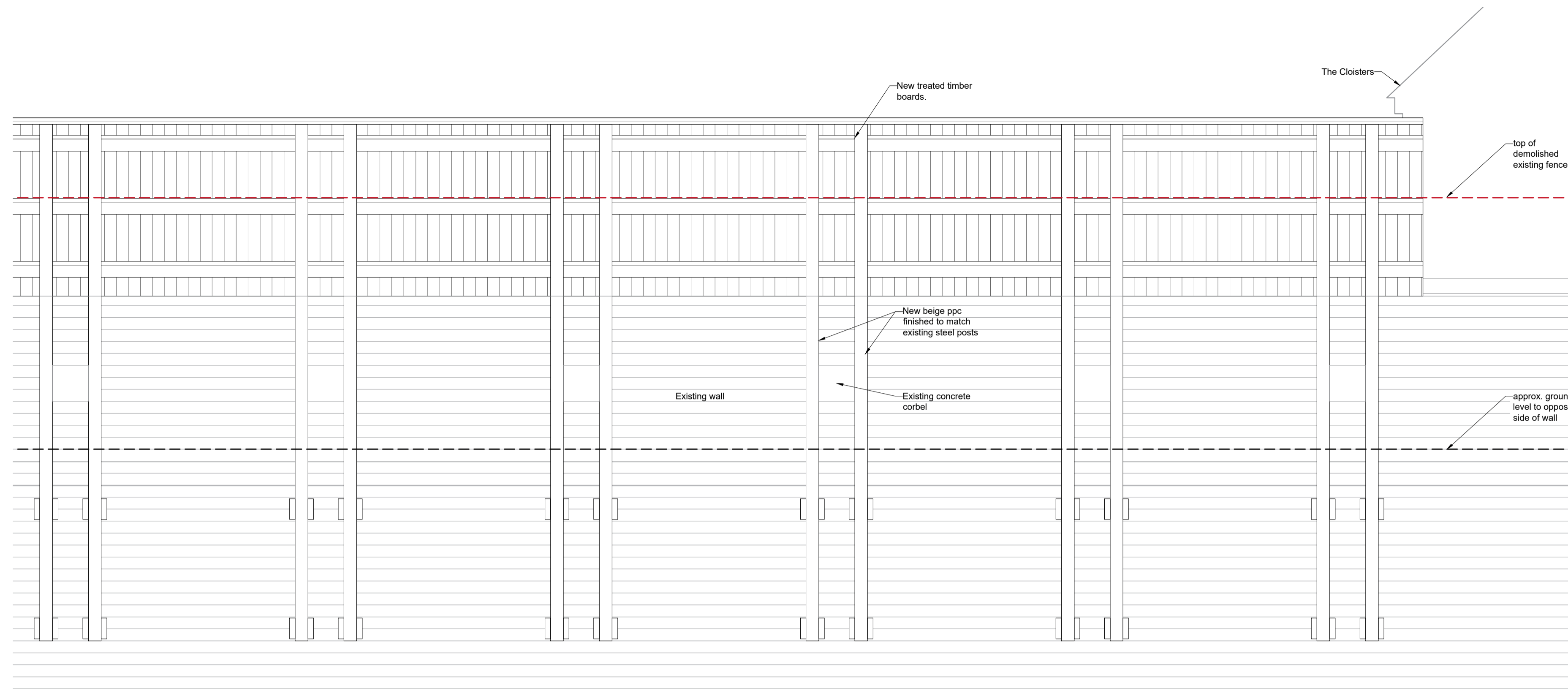
Proposed Boundary Fence Elevation from inside the site Scale 1:20
