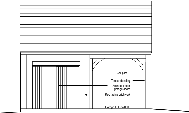
SOUTHWEST ELEVATION
