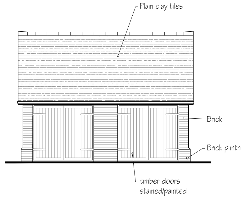
SOUTH ELEVATION 1:100
