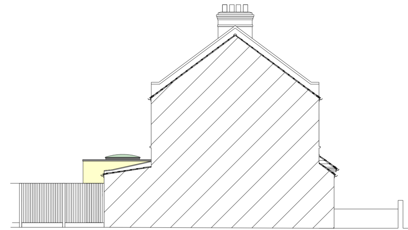
PROPOSED SIDE ELEVATION (Viewed from Number 25)
