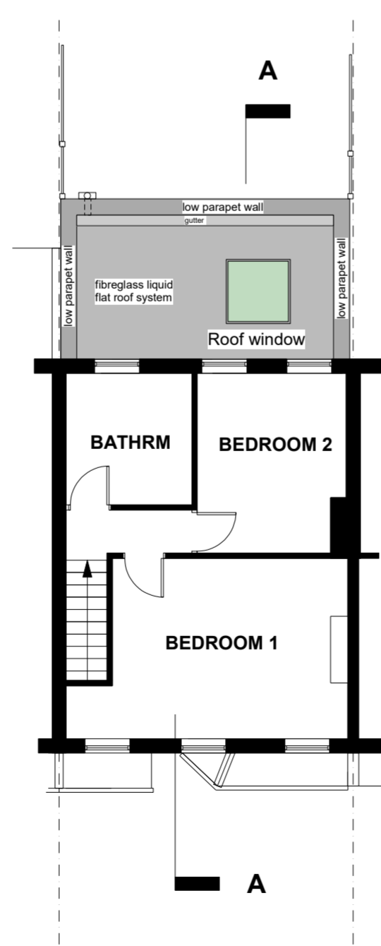
PROPOSED FIRST FLOOR AND ROOF PLAN
