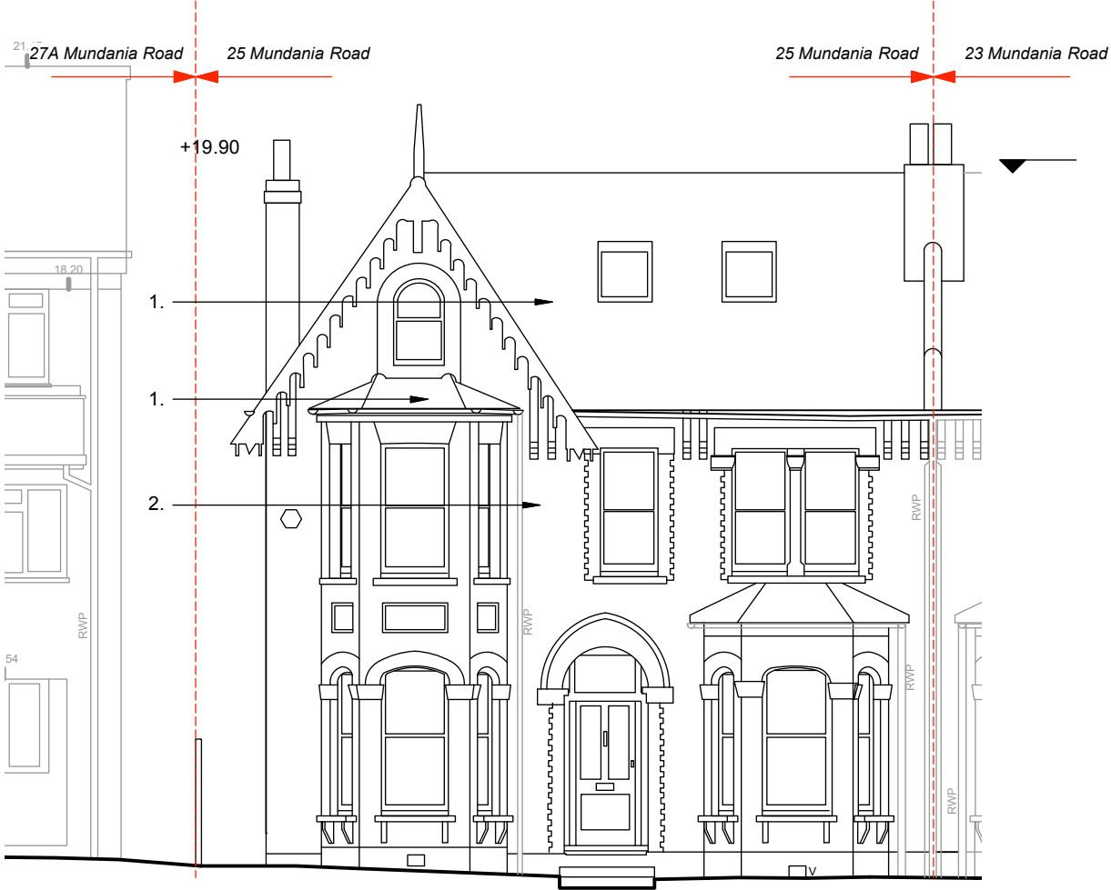
PROPOSED NORTH (FRONT) ELEVATION
