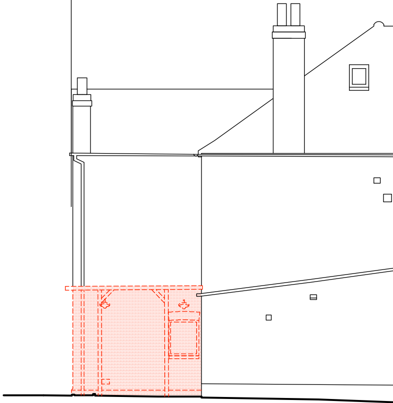
EXISTING EAST (SIDE) ELEVATION
