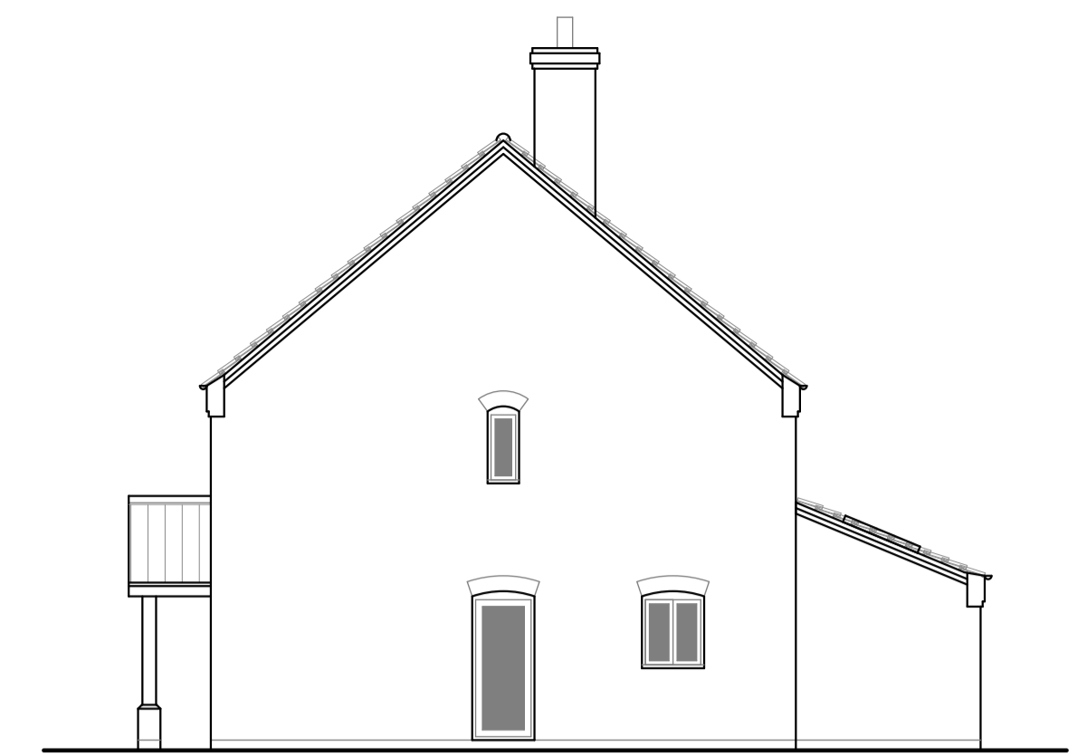
SIDE ELEVATION - EAST Scale 1:100
