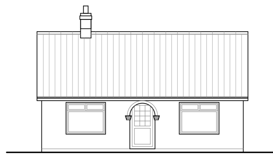
FRONT ELEVATION - SOUTH Scale 1:100
