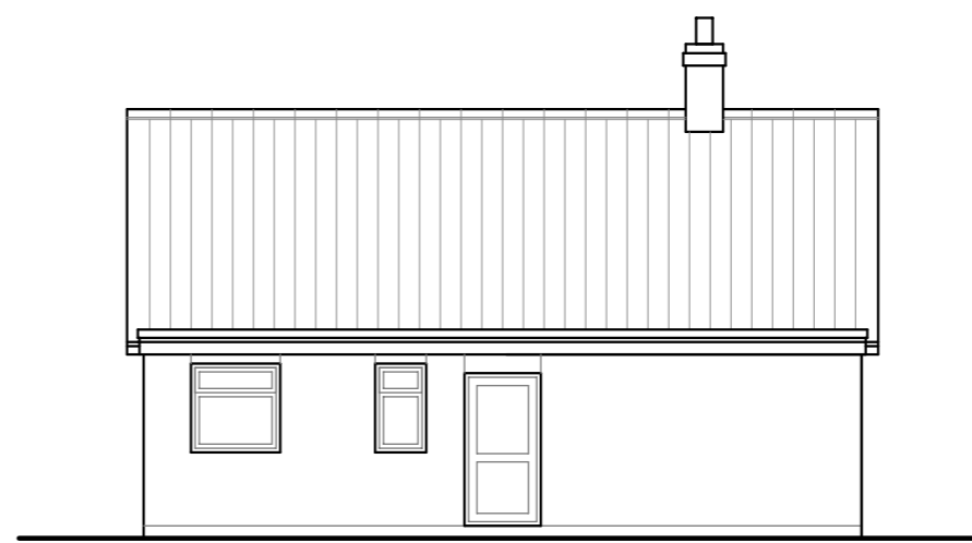
REAR ELEVATION - NORTH Scale 1:100
