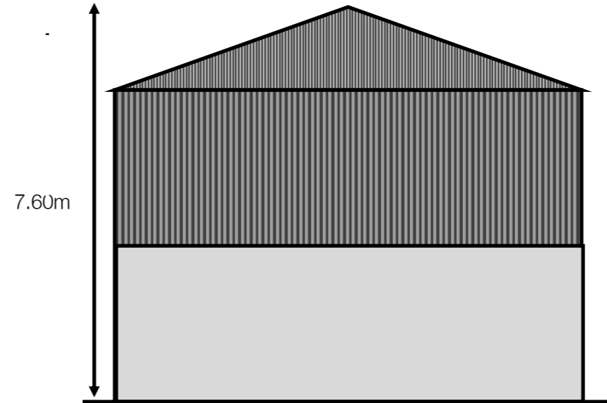
North Elevation 1:100
