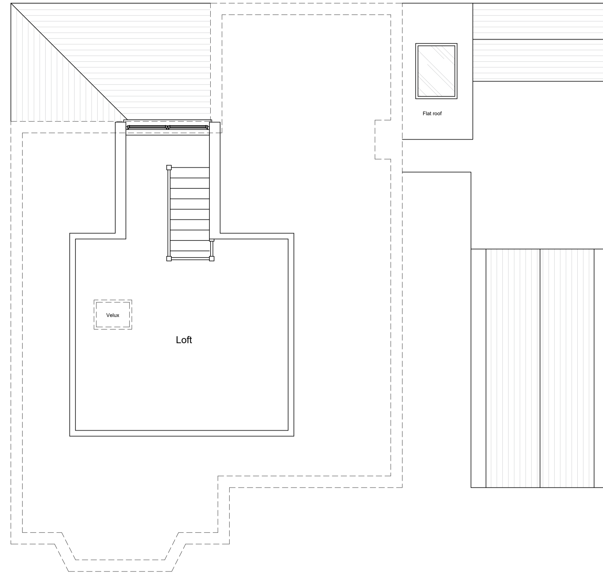
Proposed second floor Scale 1:50
