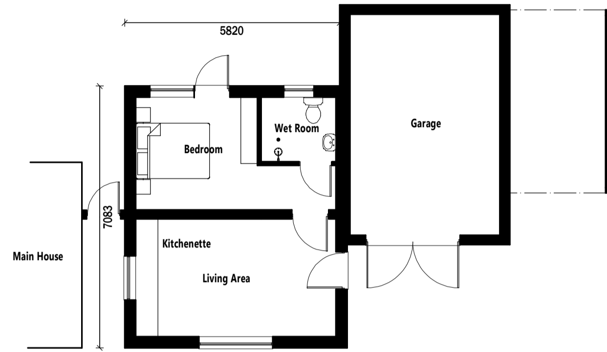
Floor Plan PROPOSED
