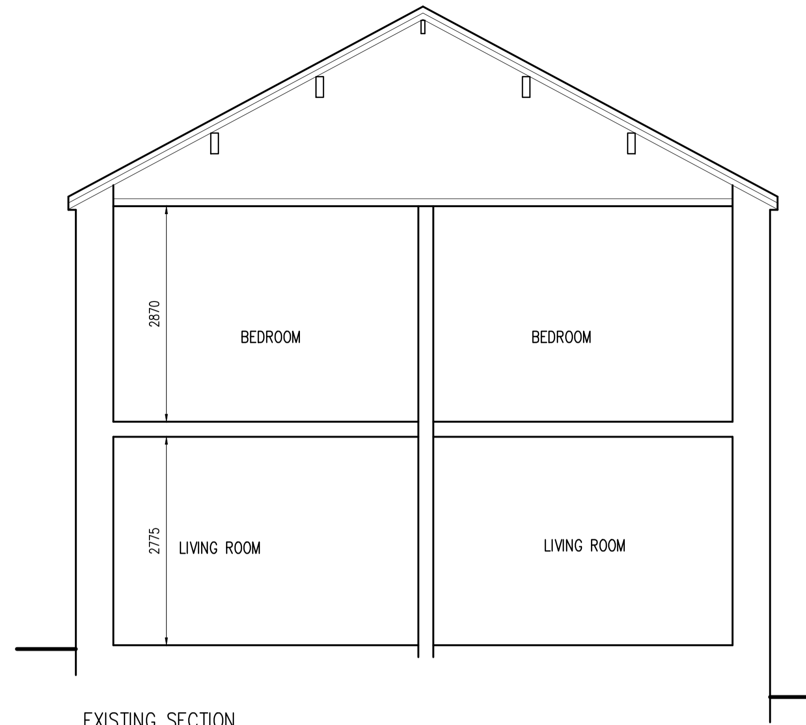
EXISTING SECTION
