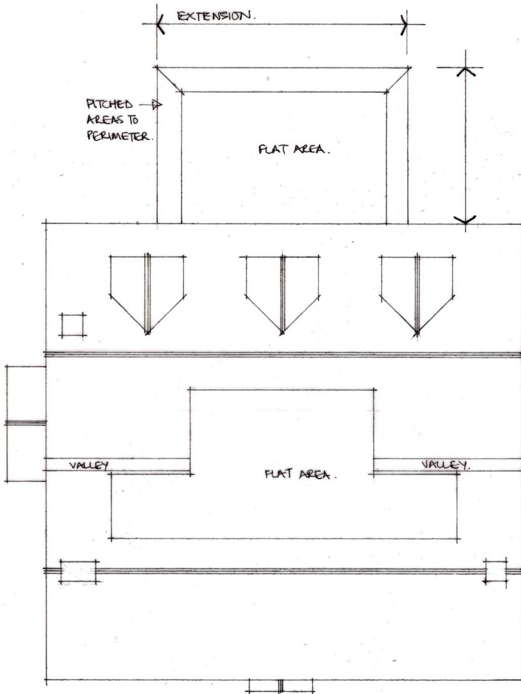
proposed roof layout. 1:100.
