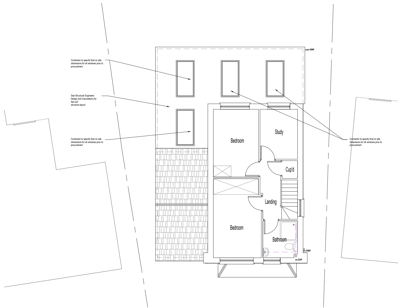
First Floor Plan Area ca. 37.26 m 2
