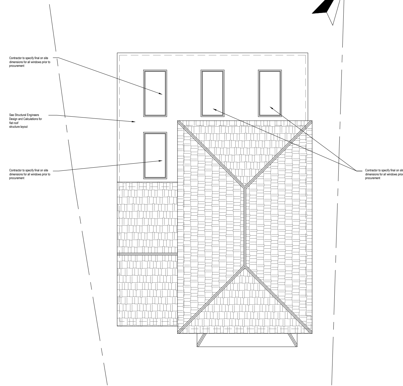
Roof Plan
